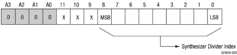
Figure 5. Divider Register (Write Only)
