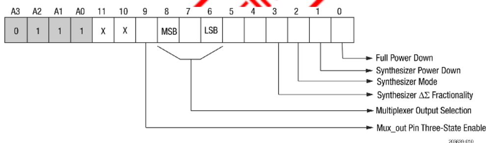
Figure 10. Power Down/Multiplexer Output Select Control Register (Write Only)
