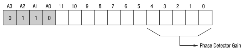
Figure 9. Phase Detector/Charge Pump Control Register (Write Only)
