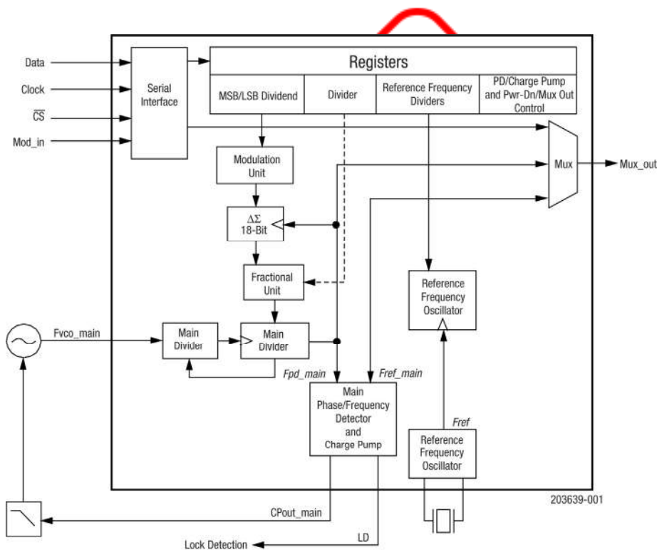
Figure 1. SKY72310-11 Functional Block Diagram
