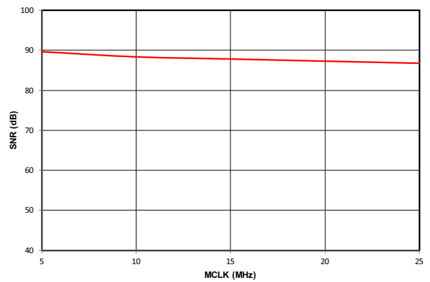
Figure 14. Si8935 Signal-to-Noise Ratio (dB) vs. MCLK (MHz)
