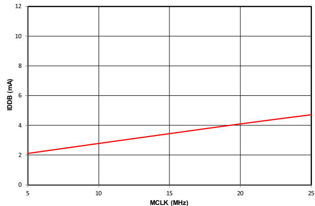
Figure 28. Si8935 IDDDB (mA) vs. MCKL (MHz)
