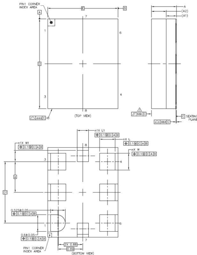
Figure 6.3. Si564 (2.5x3.2 mm) Outline Diagram
