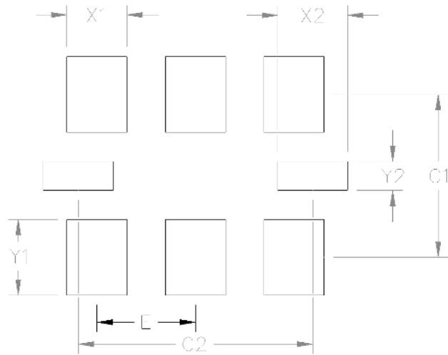
Figure 7.1. Si564 (5x7 mm) PCB Land Pattern
