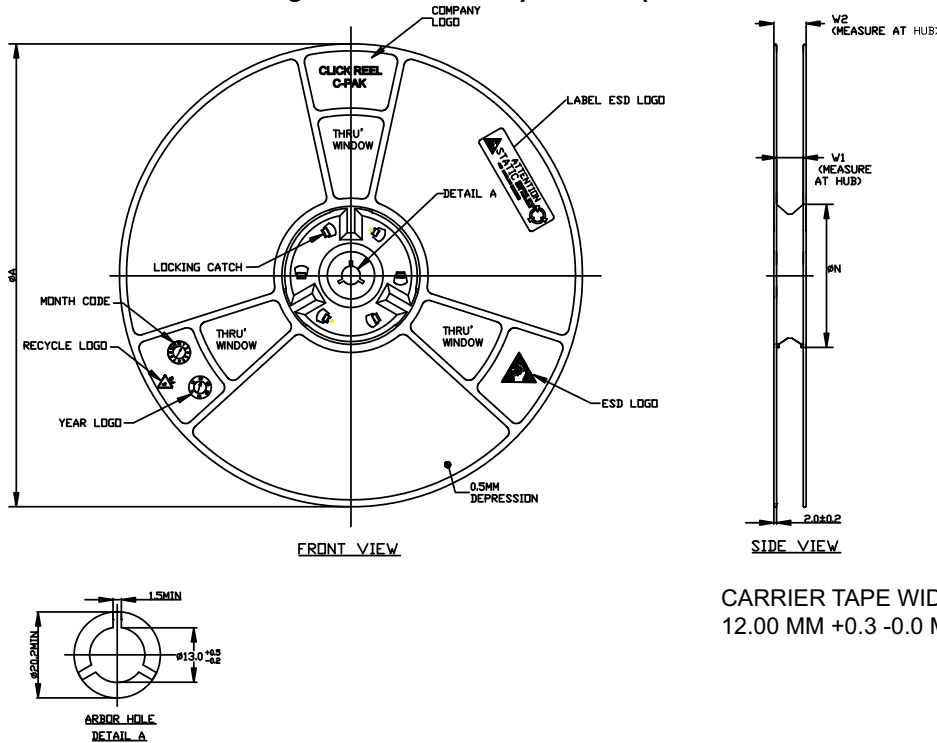
Figure 45. Narrow Body Reel Information
