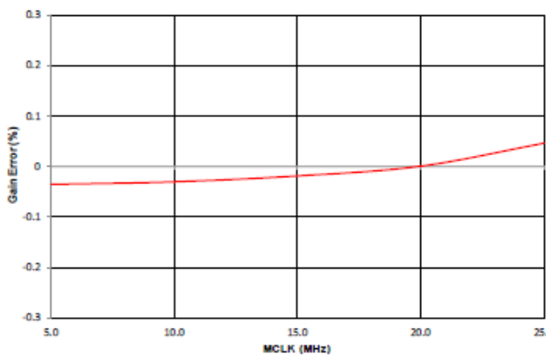
Figure 30. Si8935 Gain Error (%) vs. MCLK (MHz)
