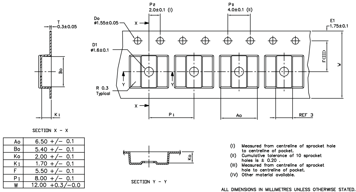
Figure 44. Narrow Body Carrier Tape Information
