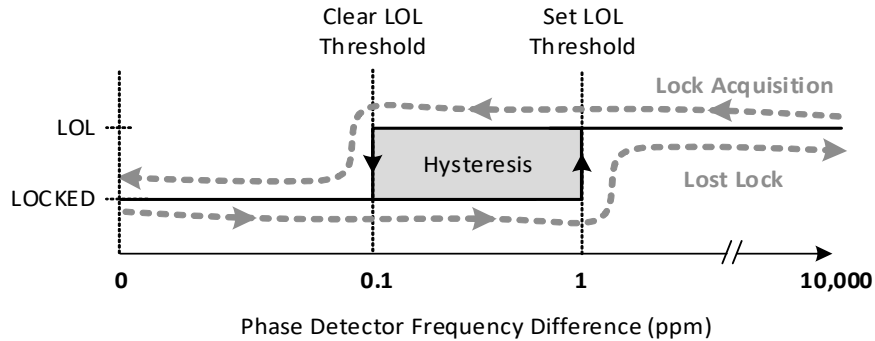
Figure 14. LOL Set and Clear Thresholds
