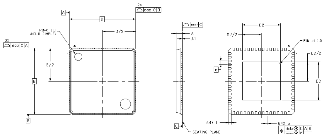
Figure 29. Si5397 A/B/C/D and Si5396 C/D (External Reference) Package Diagram
