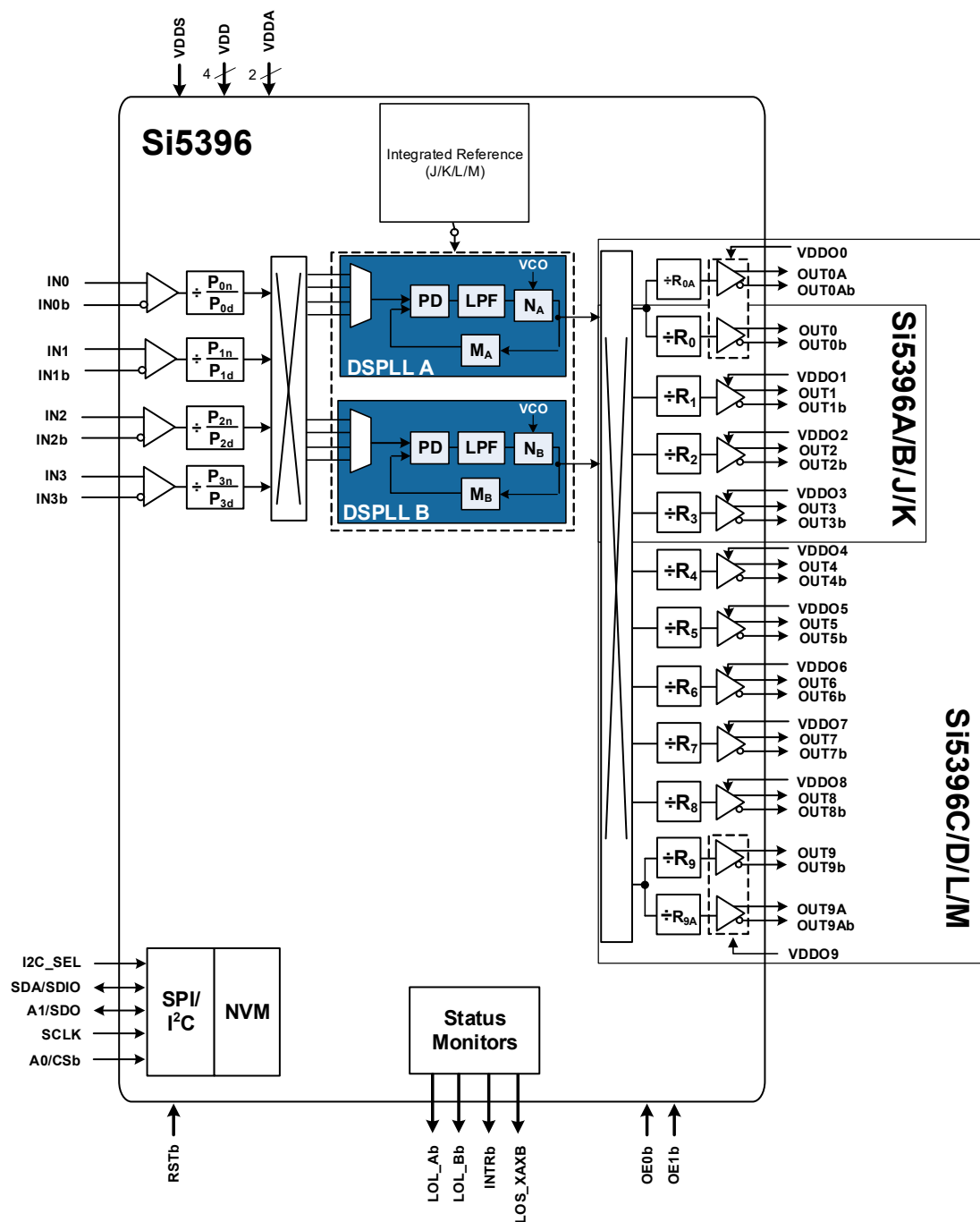
Figure 20. Si5396 Block Diagram
