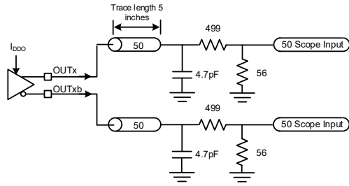
LVC MOS Output Test Configuration
