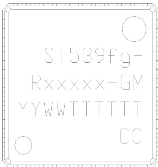
Figure 38. Si5395 A/B/C/D/P QFN 9x9 mm Package
