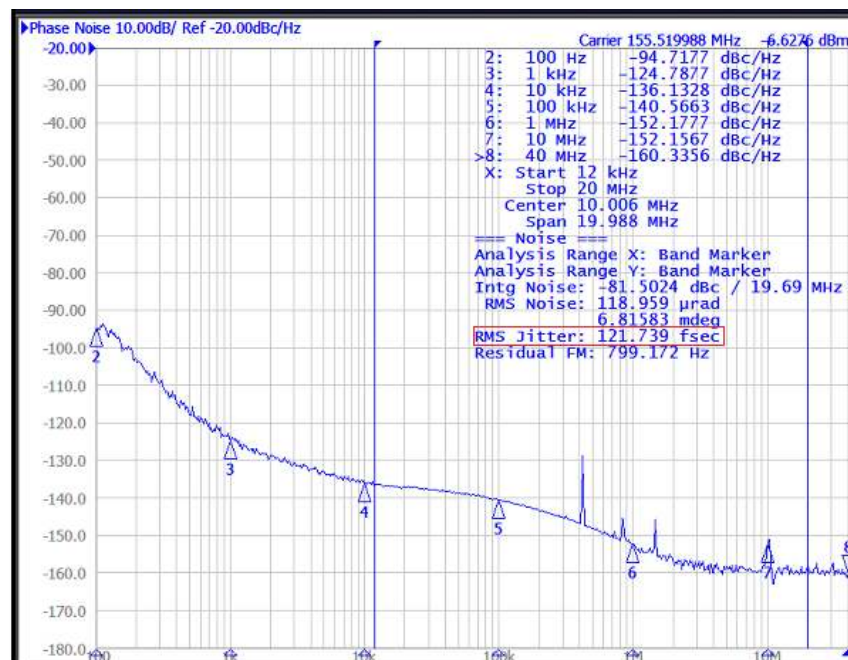
Figure 29. Input = 25 MHz; Output = 155.52 MHz, 2.5 V LVDS (Fractional Mode)
