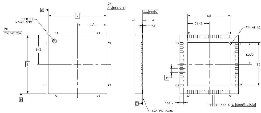
Figure 35. Si5394 and Si5392 A/B/C/D/P (External Reference) Package Diagram
