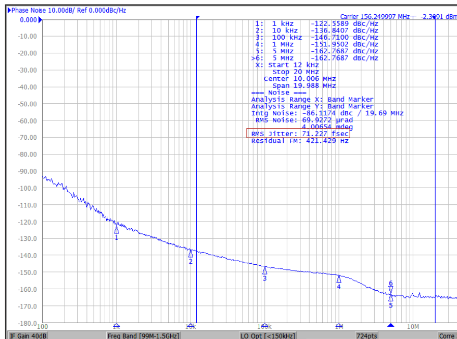
Figure 27. Input = 25 MHz; Output = 156.25 MHz, 2.5 V LVDS (Si539x E-Grade)
