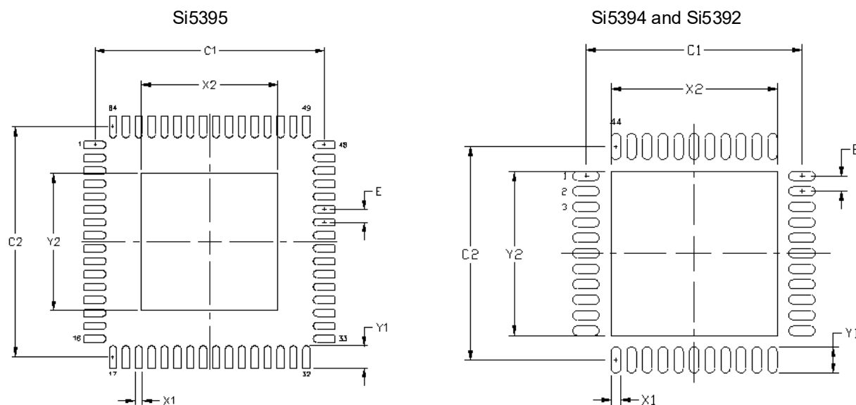
Figure 37. Si5395, Si5394, Si5392 PCB Land Patterns
