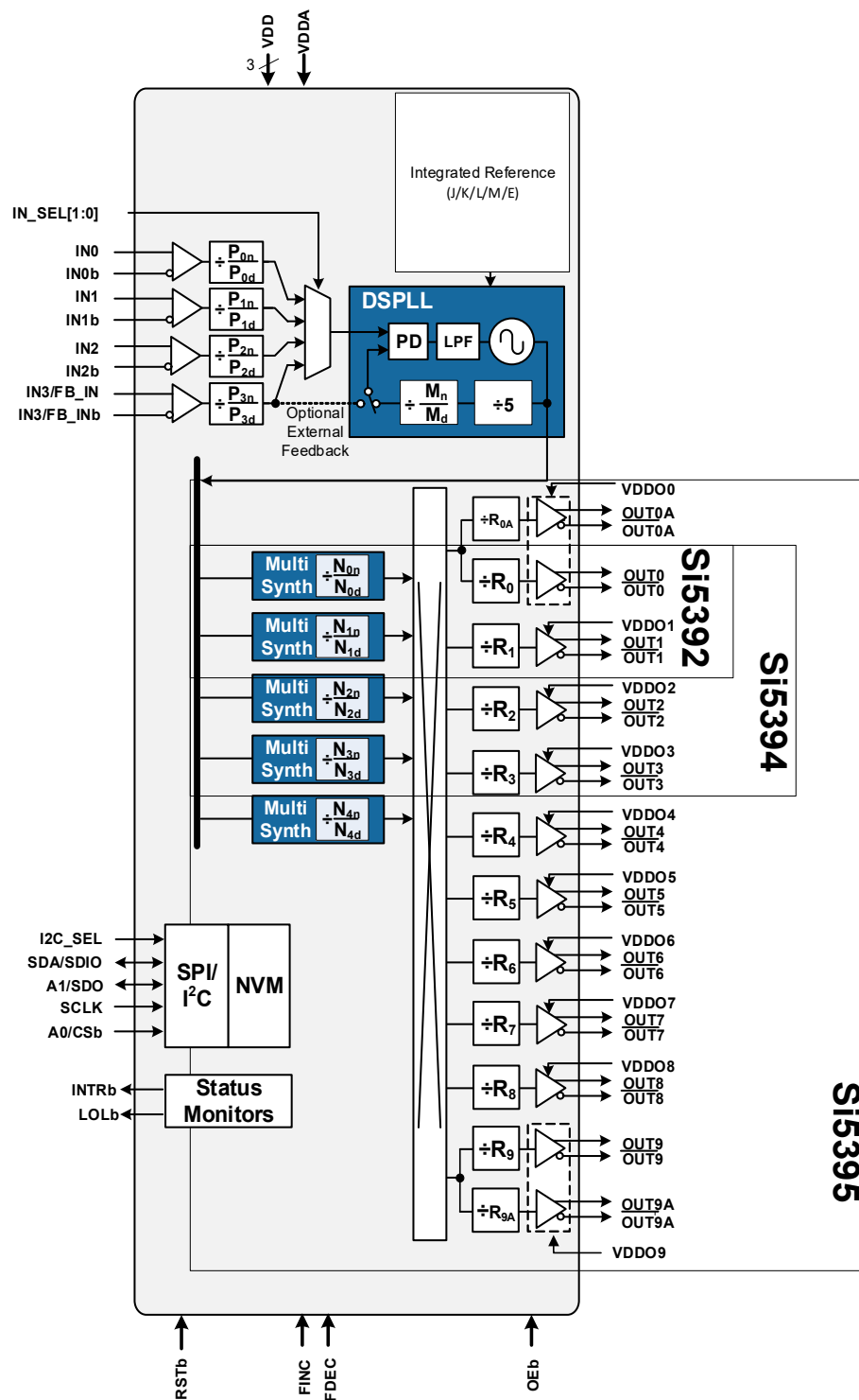
Figure 25. Si5395, Si5394, Si5392 Block Diagram
