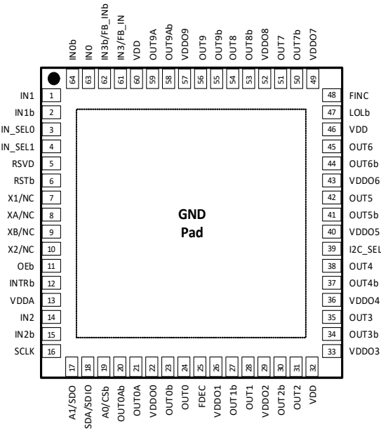
Figure 30. Si5395 (64-QFN and 64-LGA) Top View
