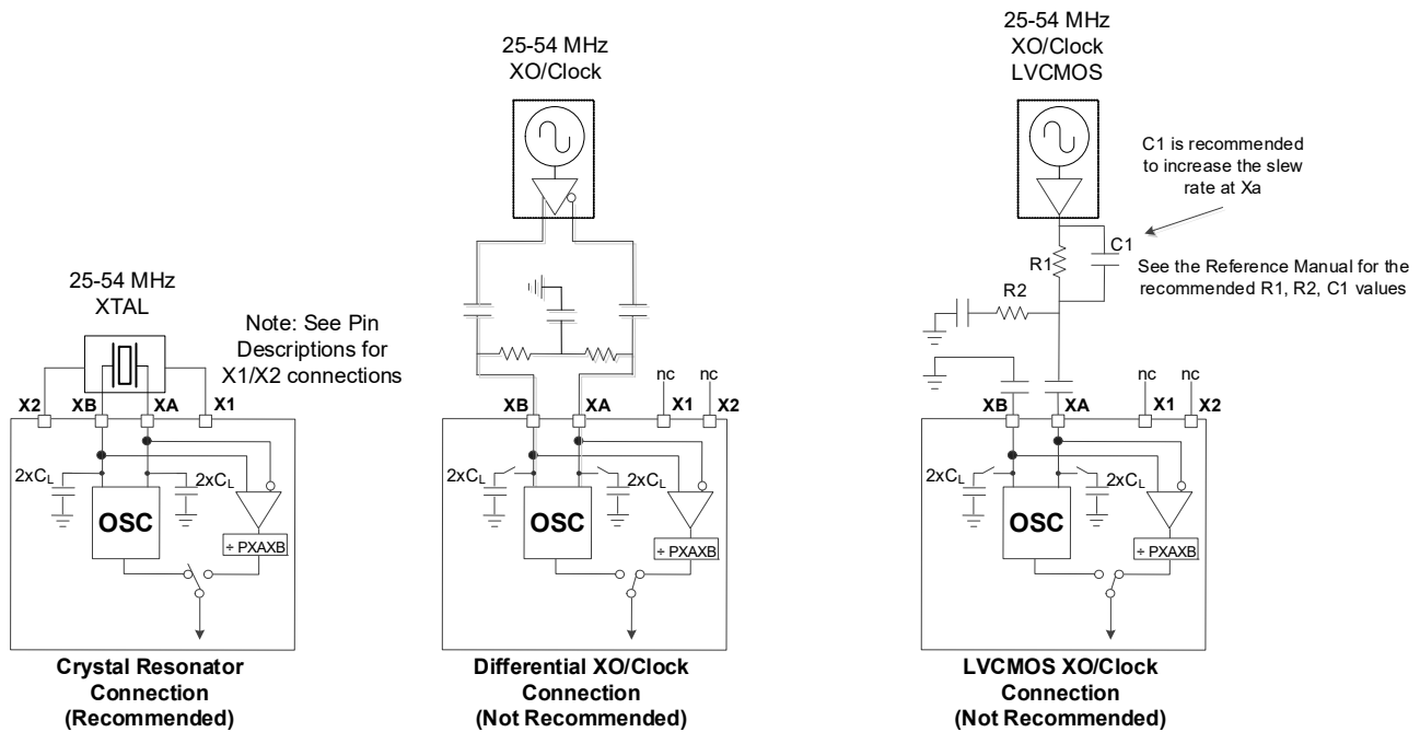
Figure 5. Crystal Resonator and External Reference Clock Connection Options
