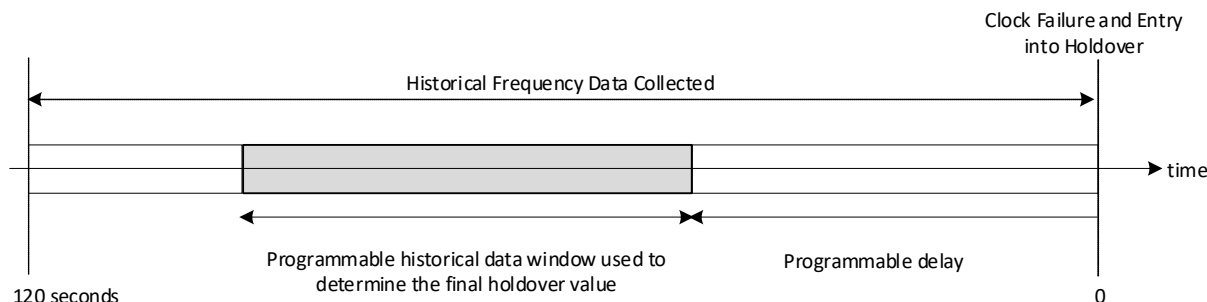
Figure 4. Programmable Holdover Window
