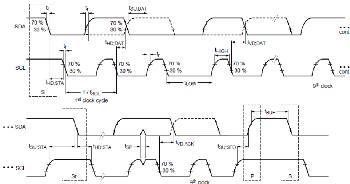
Figure 20. I 2 C Serial Port Timing Standard and Fast Modes
