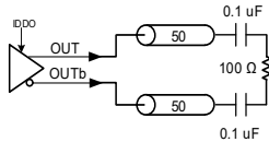
Differential Output Test Configuration
