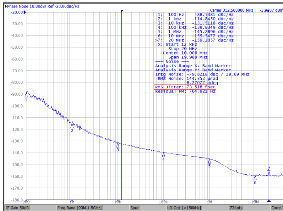
Figure 28. Input = 25 MHz; Output = 312.5 MHz, 2.5 V LVDS (Integer Mode)
