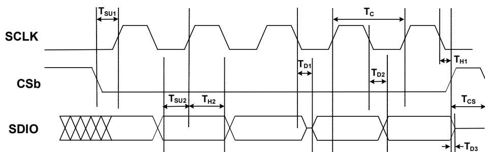
Figure 22. 3-Wire SPI Serial Interface Timing
