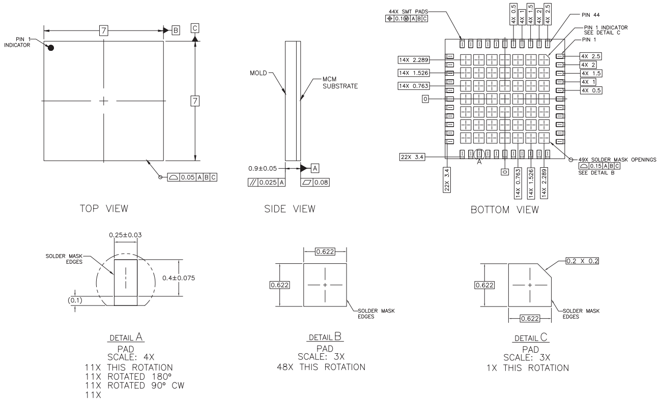
Figure 36. Si5394 and Si5392 J/K/L/M/E (Internal Reference) Package
