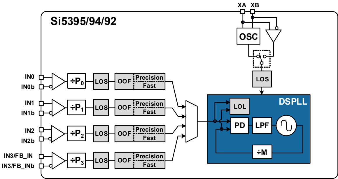
Figure 9. Si5395, Si5394, Si5392 Fault Monitors
