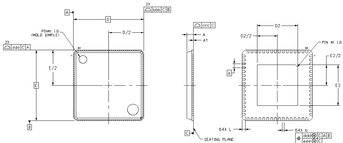
Figure 33. Si5395 A/B/C/D/P (External Reference) Package Diagram
