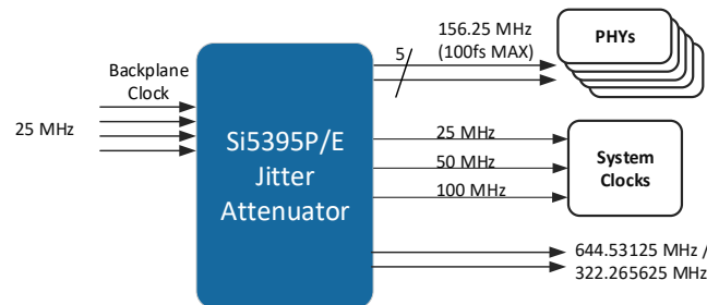
Figure 16. Si5395P/E Typical 56G SerDes Application (up to 3 domains)
