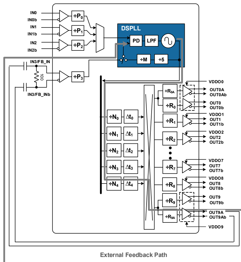
Figure 19. Si5395 Zero Delay Mode Setup
