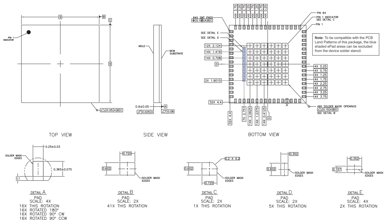
Figure 34. Si5395 J/K/L/M/E (Internal Reference) Package Diagram
