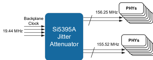
Figure 15. Si5395 A/B/C/D and J/K/L/M Jitter Attenuator
