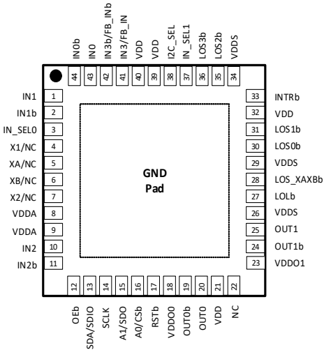
Figure 32. Si5392 (44-QFN and 44-LGA) Top View
