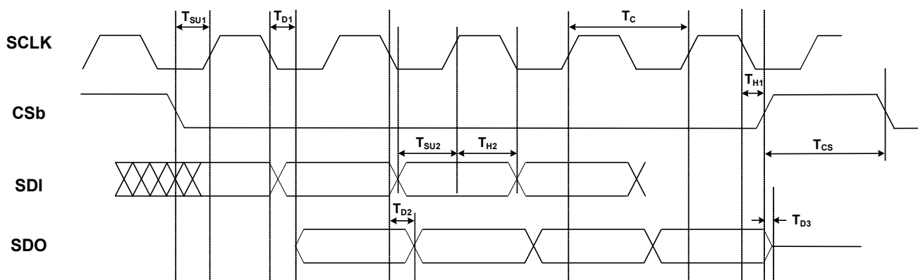
Figure 21. 4-Wire SPI Serial Interface Timing
