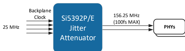
Figure 18. Si5392P/E Typical 56G SerDes Application (1 domain)
