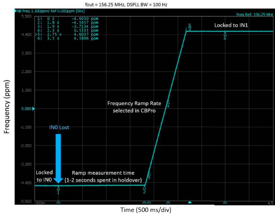
Figure 7. Output Frequency Transient — Ramped Switching Between Two 8 kHz Inputs (±4.6 ppm Offset)
