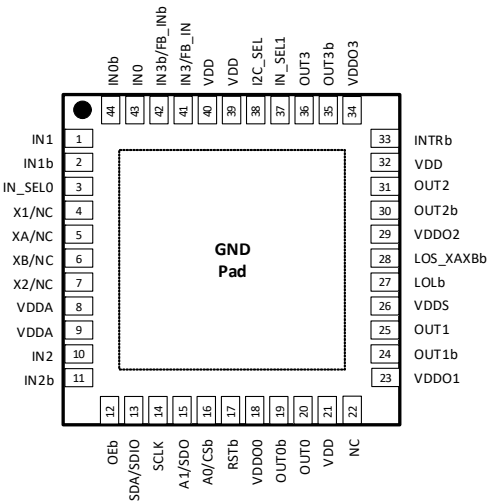
Figure 31. Si5394 (44-QFN and 44-LGA) Top View
