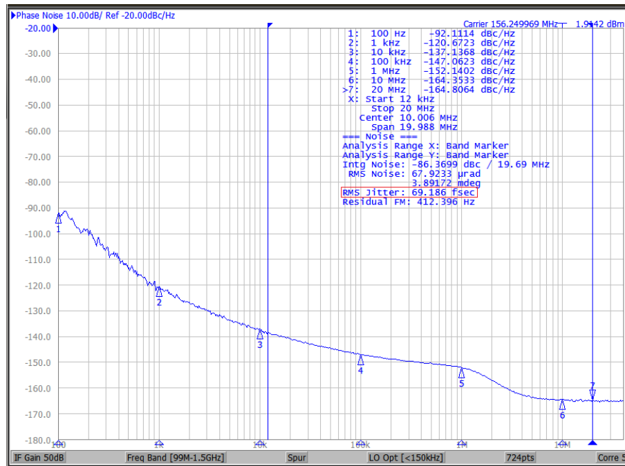
Figure 26. Input = 25 MHz; Output = 156.25 MHz, 2.5 V LVDS (Si539x P-Grade)
