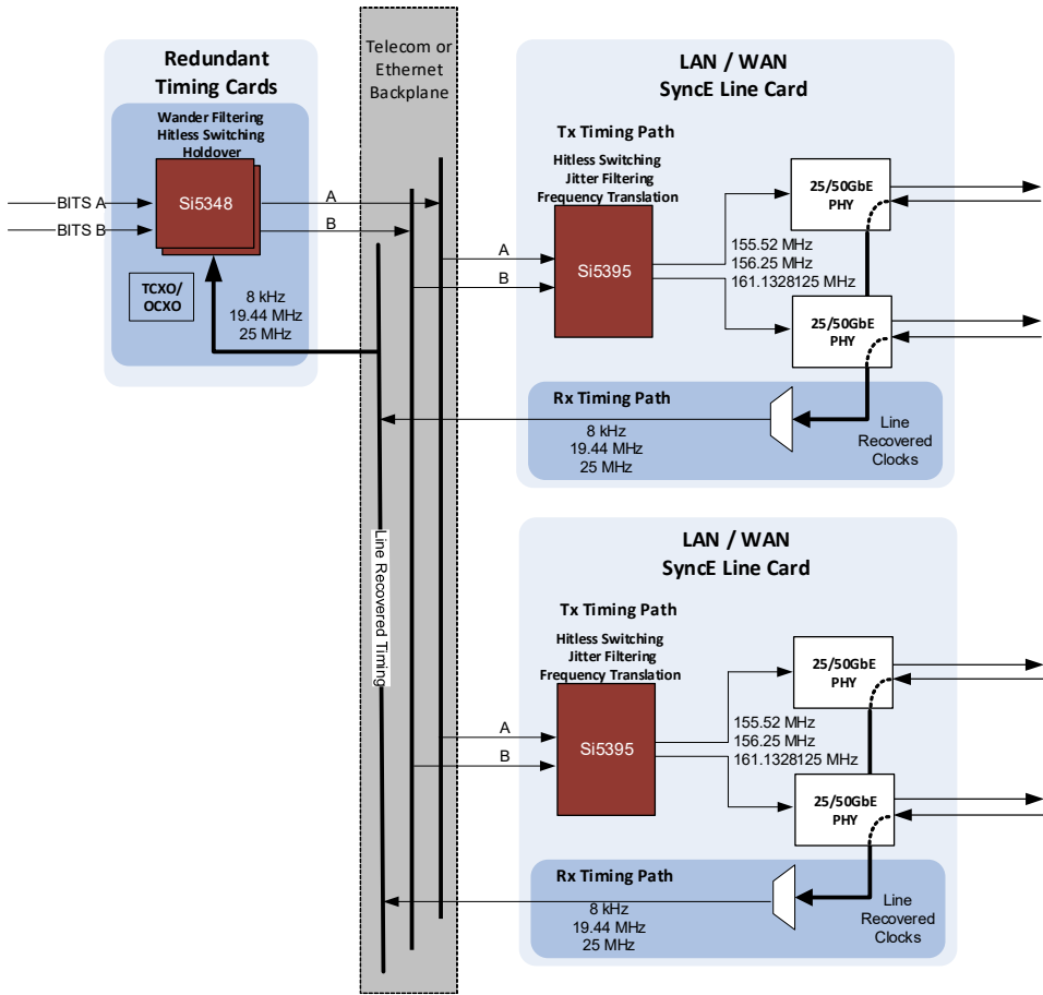
Figure 24. SyncE Line Card
