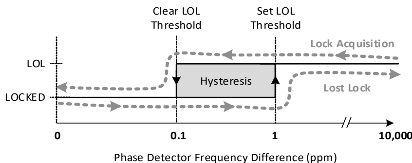
Figure 14. LOL Set and Clear Thresholds
