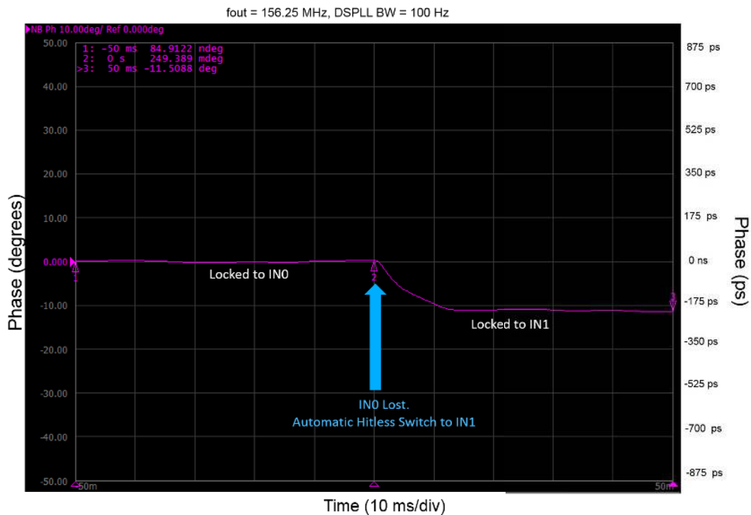
Figure 6. Output Phase Transient — Hitless Switching Between Two 25 MHz Inputs (0 ppm, 180 Degree Phase Shift)
