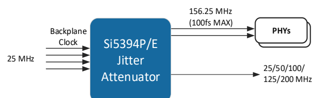
Figure 17. Si5394P/E Typical 56G SerDes Application (up to 2 domains)
