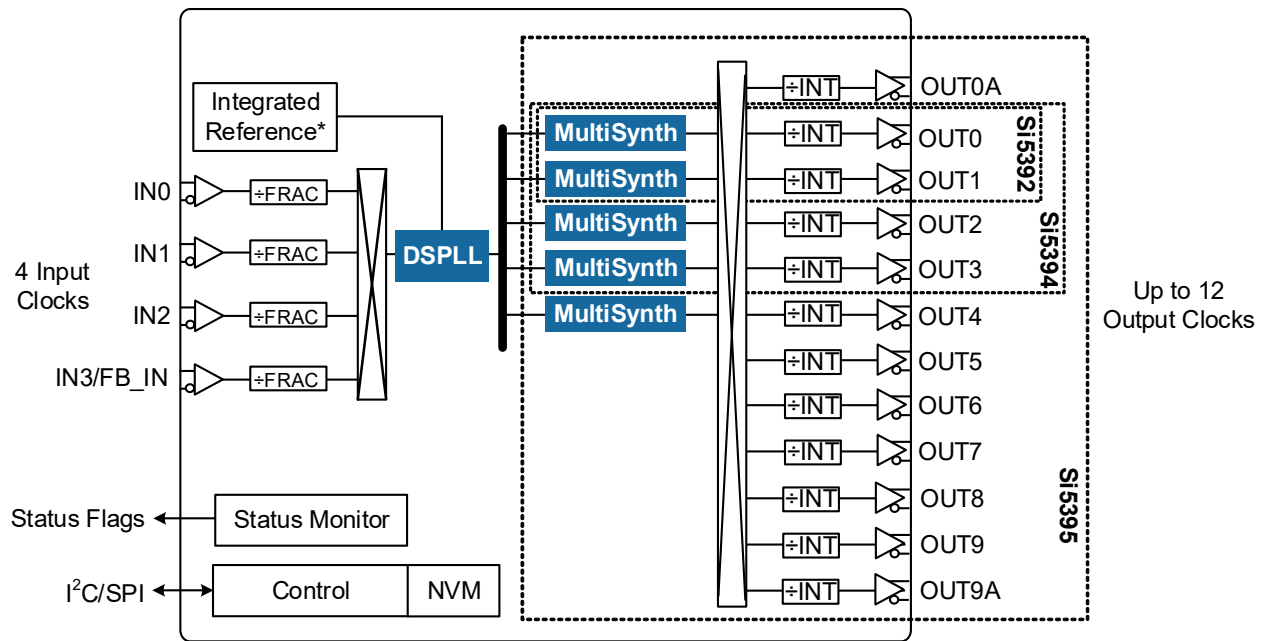
Figure 1. Si5395, Si5394, Si5392
