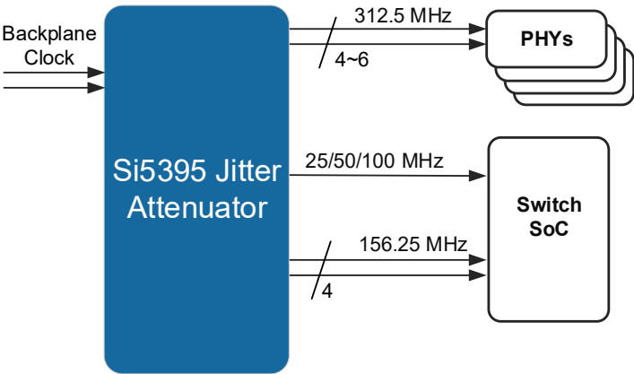
Figure 23. Typical 56G SerDes Application
