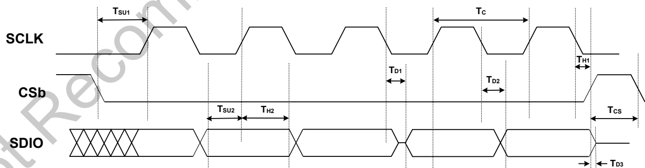
Figure 5.3. 3-Wire SPI Serial Interface Timing
