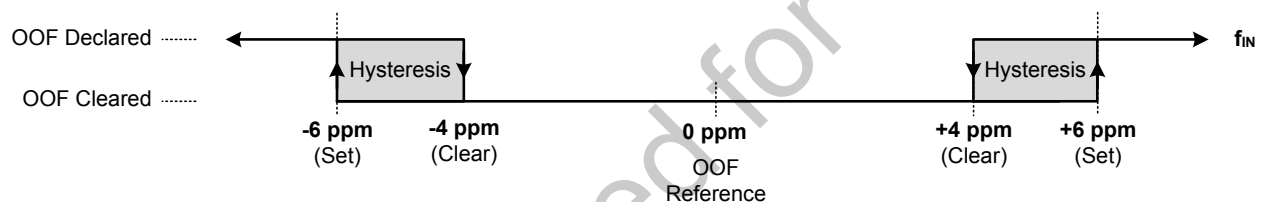
Figure 3.9. Example of Precise OOF Monitor Assertion and De-assertion Triggers
