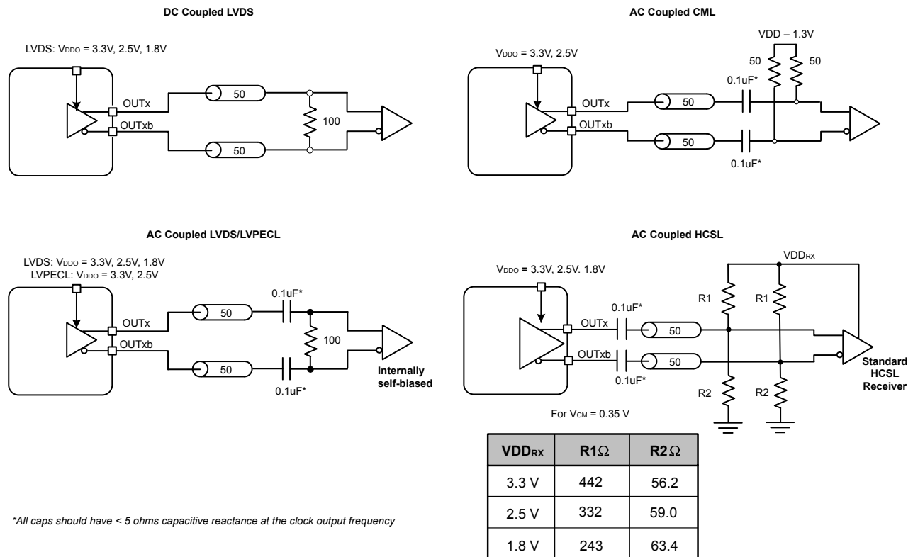
Figure 5.1. Supported Differential Output Terminations
