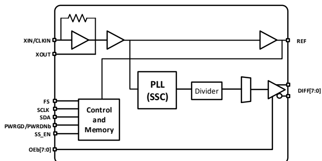
Figure 2. Si52208 Block Diagram 8-Output, 48-QFN
