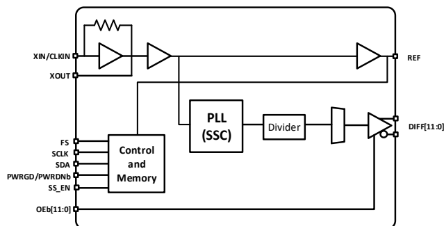
Figure 1. Si52212 Block Diagram 12-Output, 64-QFN
