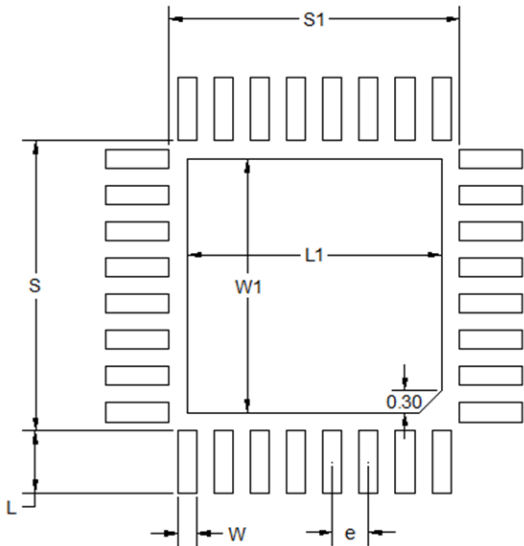
Figure 32. Si52204 Land Pattern
