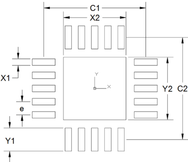
Figure 35. Si52202 Land Pattern
