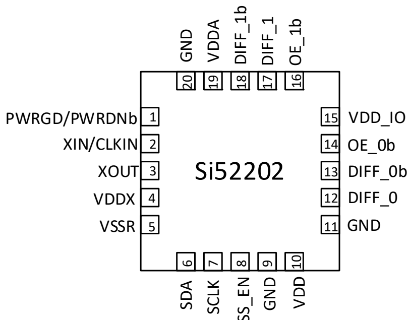
Figure 8. Si52202 20-pin QFN Pinout
