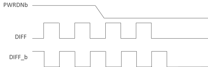
Figure 13. PWRDNb Assertion
