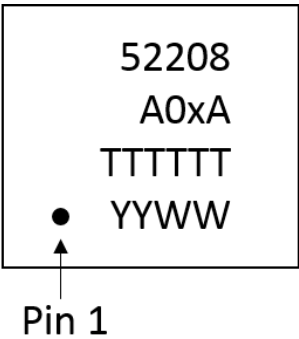
Figure 30. Si52208 Top Marking
