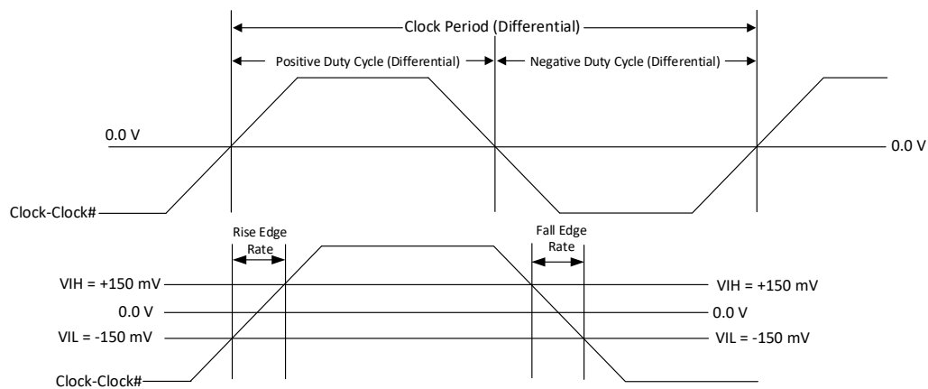
Figure 18. Differential Output Signals (for AC Parameters Measurement)
