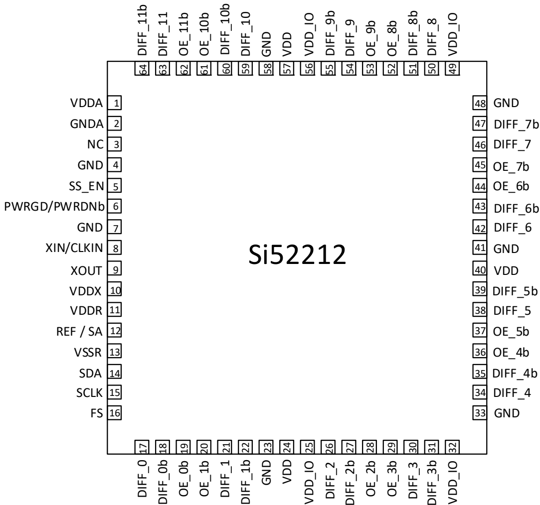
Figure 5. Si52212 64-Pin QFN Pinout
