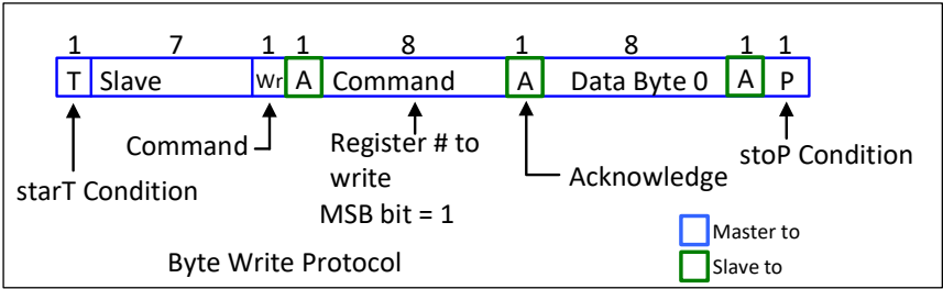
Figure 24. Byte Write Protocol
