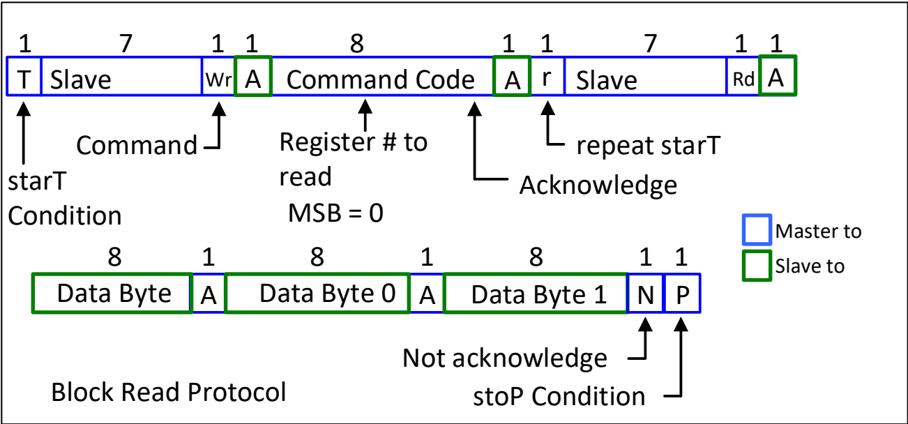
Figure 21. Block Read Protocol
