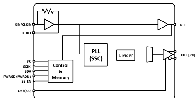
Figure 3. Si52204 Block Diagram 4-Output, 32-QFN
