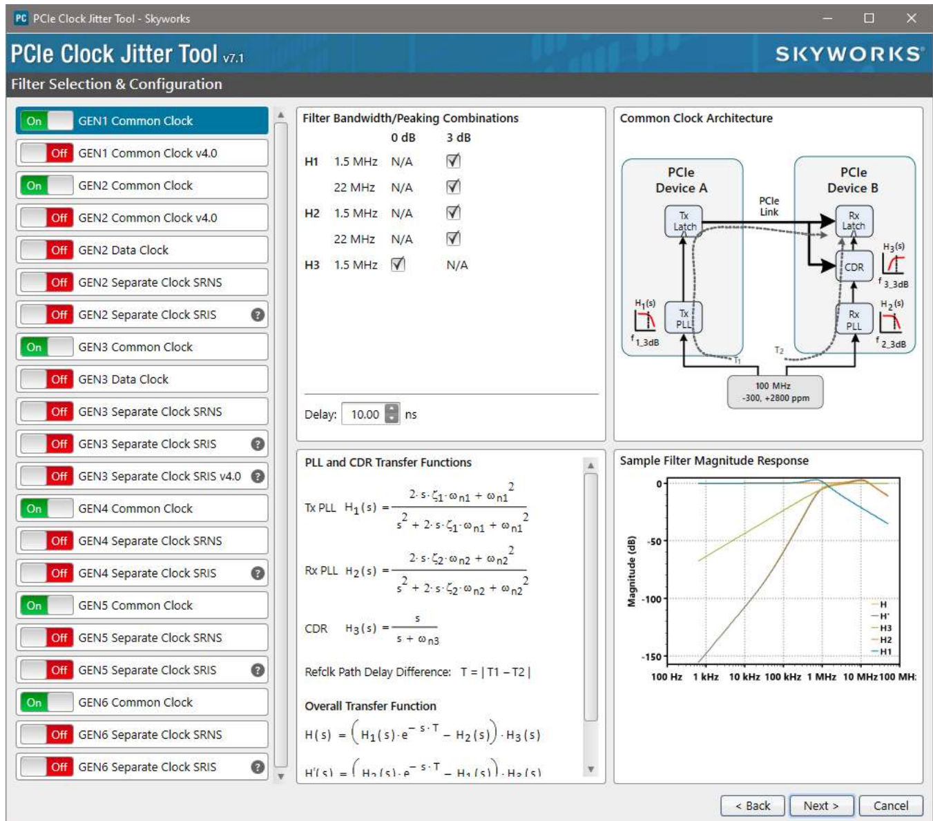
Figure 20. PCIe Clock Jitter Tool
