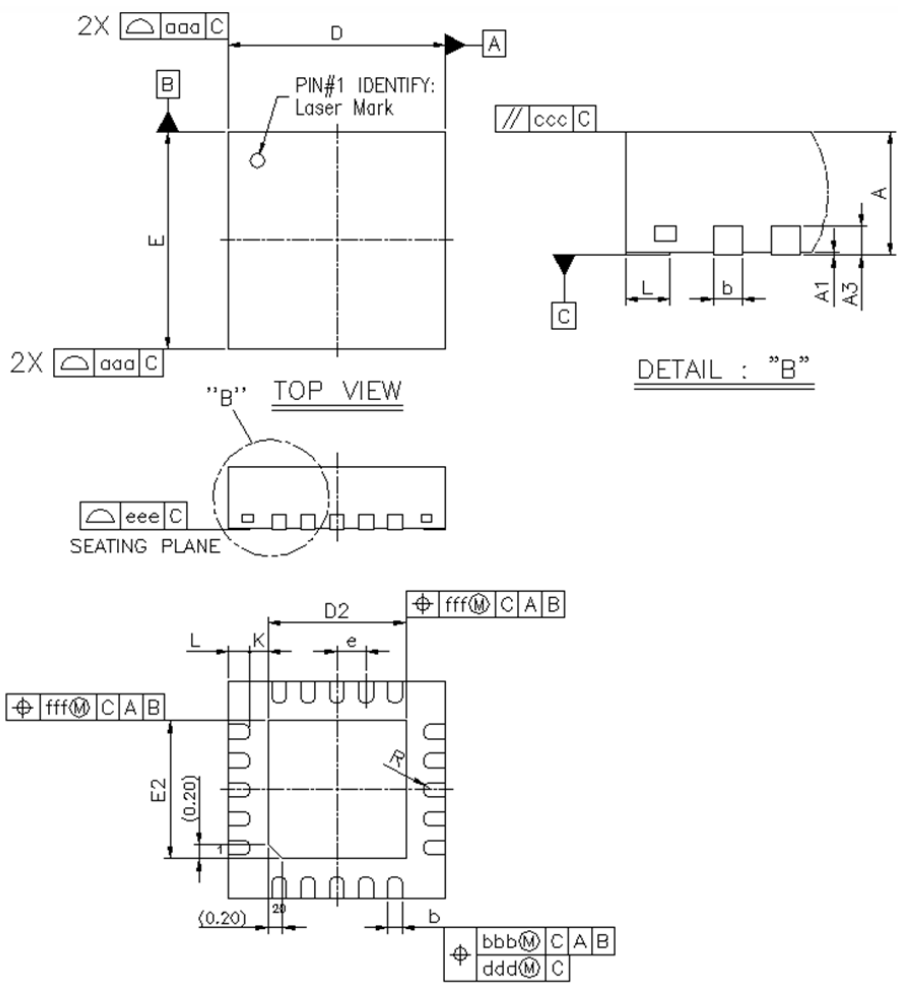
Figure 34. Si52202 Package Diagram
