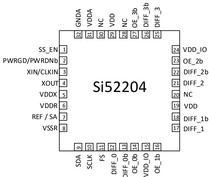
Figure 7. Si52204 32-pin QFN Pinout
