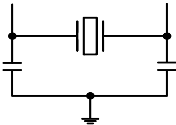
Figure 9. Crystal Capacitive Clarification
