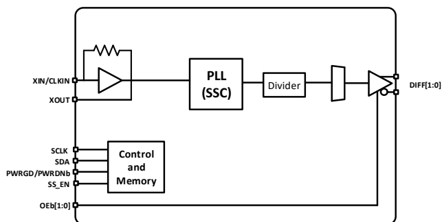
Figure 4. Si52202 Block Diagram 2-Output, 20-QFN
