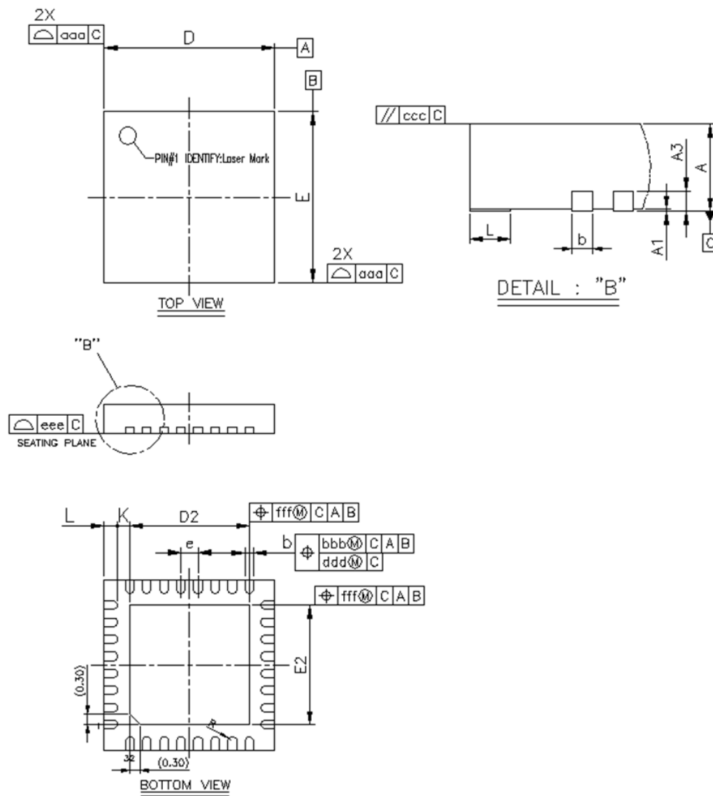
Figure 31. Si52204 Package Diagram
