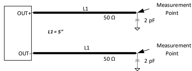
Figure 17. 0.7 V Differential Load Configuration
