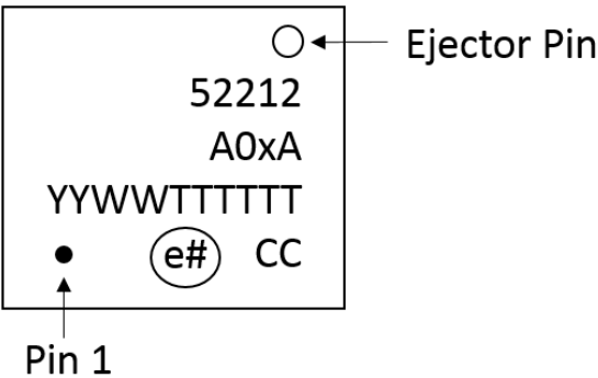
Figure 27. Si52212 Top Marking
