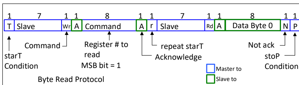
Figure 23. Byte Read Protocol
