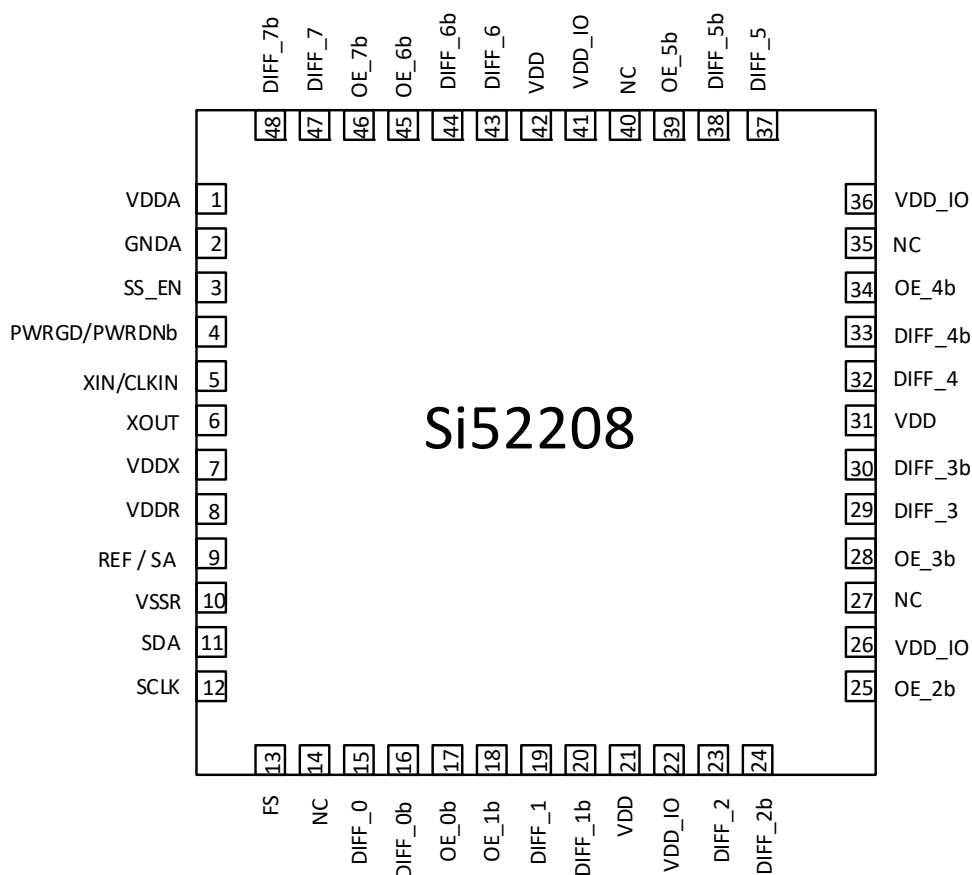
Figure 6. Si52208 48-pin QFN Pinout
