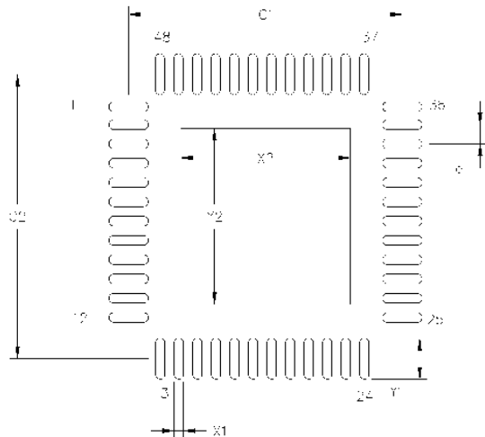
Figure 29. Si52208 Land Pattern
