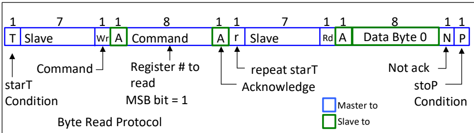
Figure 23. Byte Read Protocol
