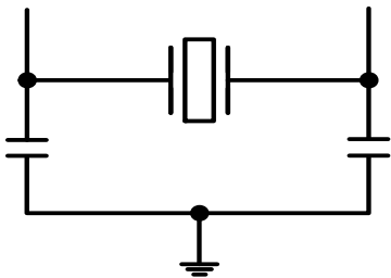
Figure 9. Crystal Capacitive Clarification
