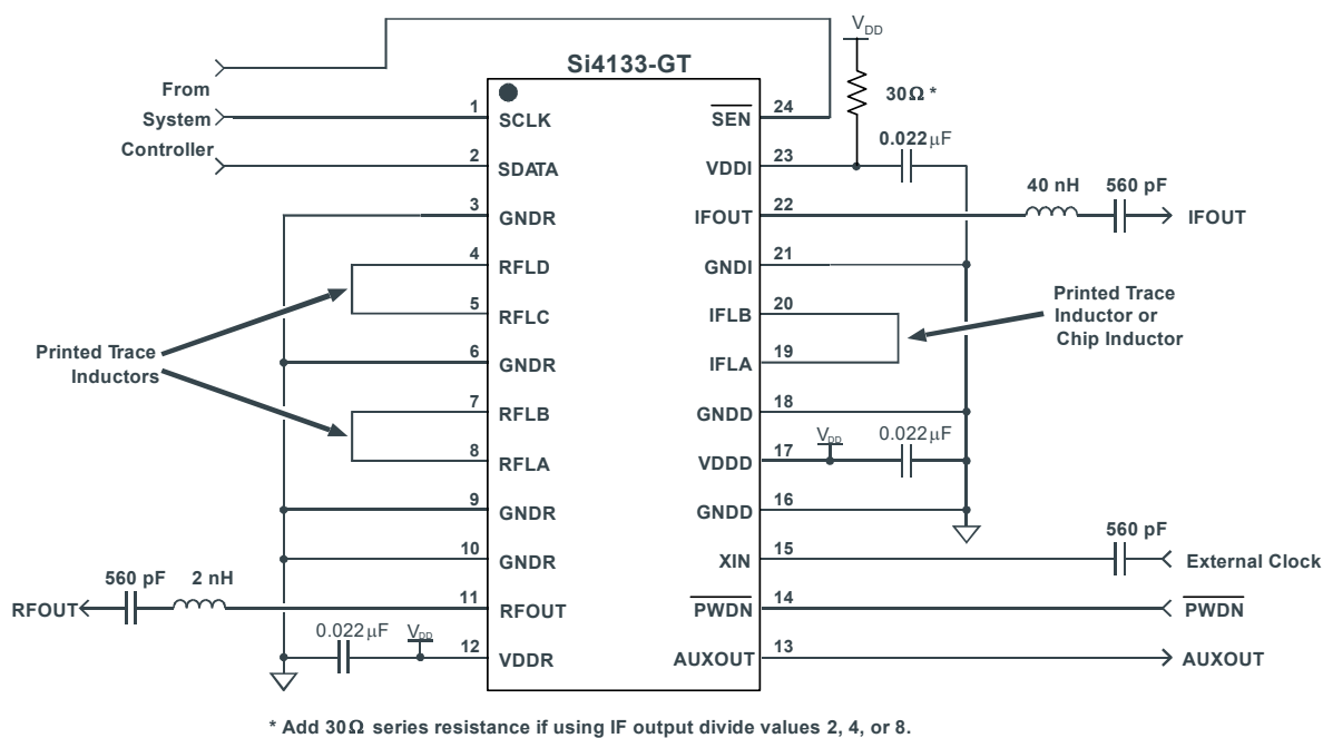
Figure 13. Si4133-GT
