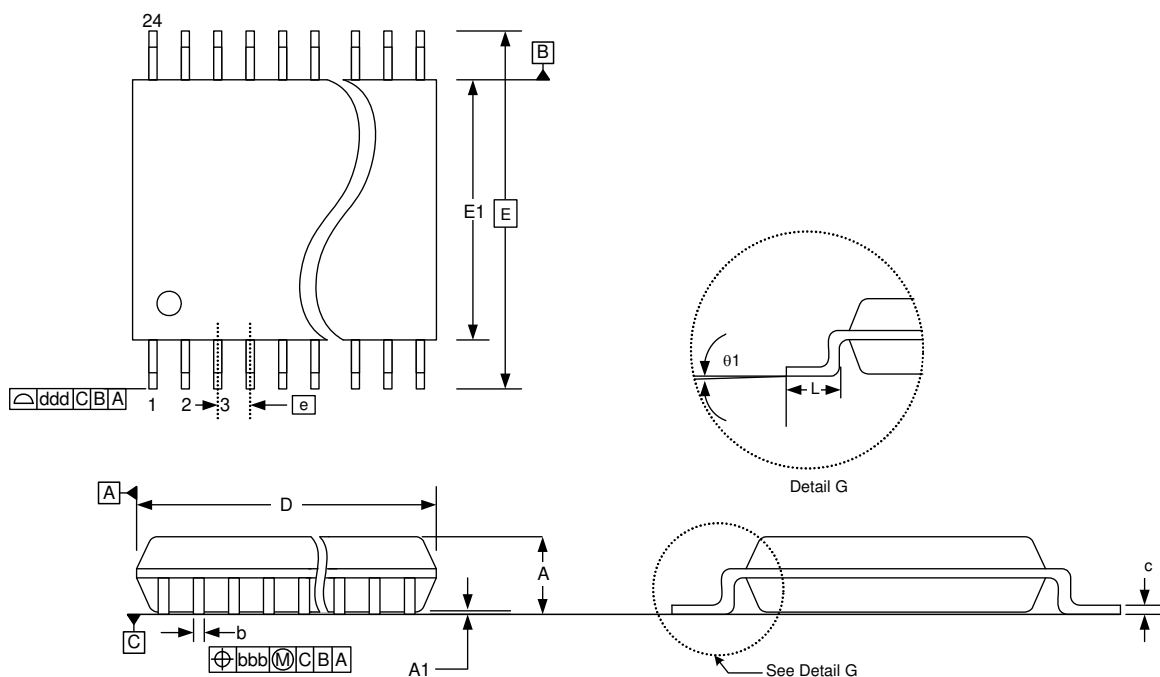
Figure 19. 24-Pin Thin Shrink Small Outline Package (TSSOP)
