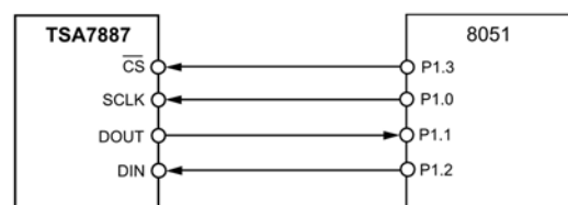
Figure 19: Interfacing the TSA7887 to Legacy 8051-type Microcontrollers.
