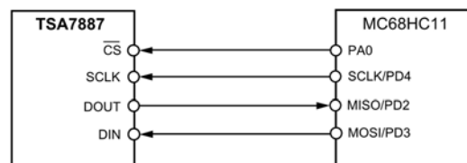
Figure 18: Interfacing the TSA7887 to 68HC11-type Microcontrollers.
