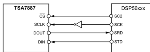
Figure 17: Interfacing the TSA7887 to DSP56xxx-type DSPs.
