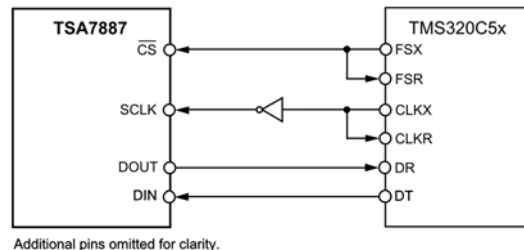
Figure 15: Interfacing the TSA7887 to TMS320C5x-type DSPs.
