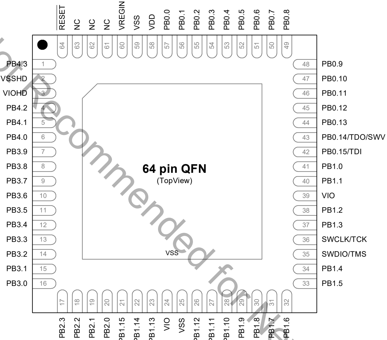
Figure 6.4. SiM3C1x6-GM Pinout
