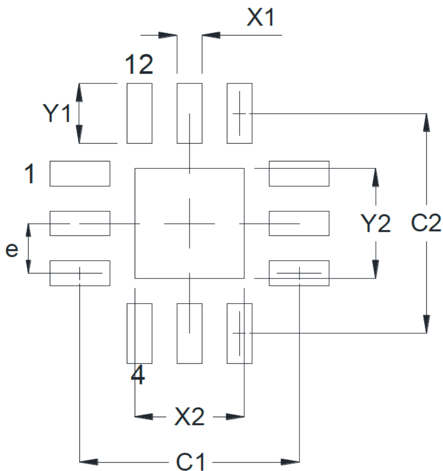
Figure 9.2. QFN12 PCB Land Pattern Drawing
