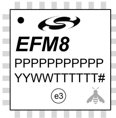
Figure 9.3. Package Marking
