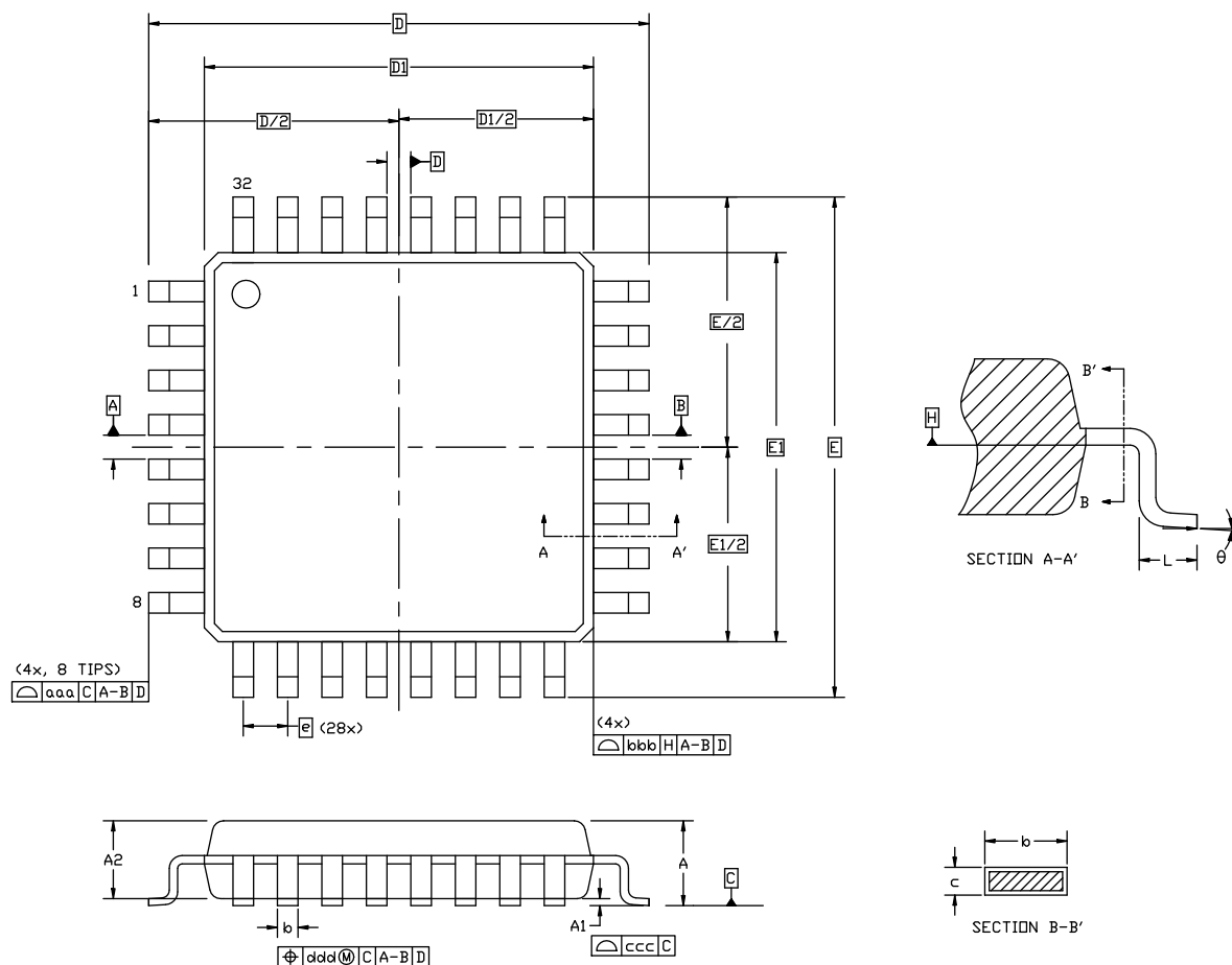
Figure 9.1. Package Drawing
