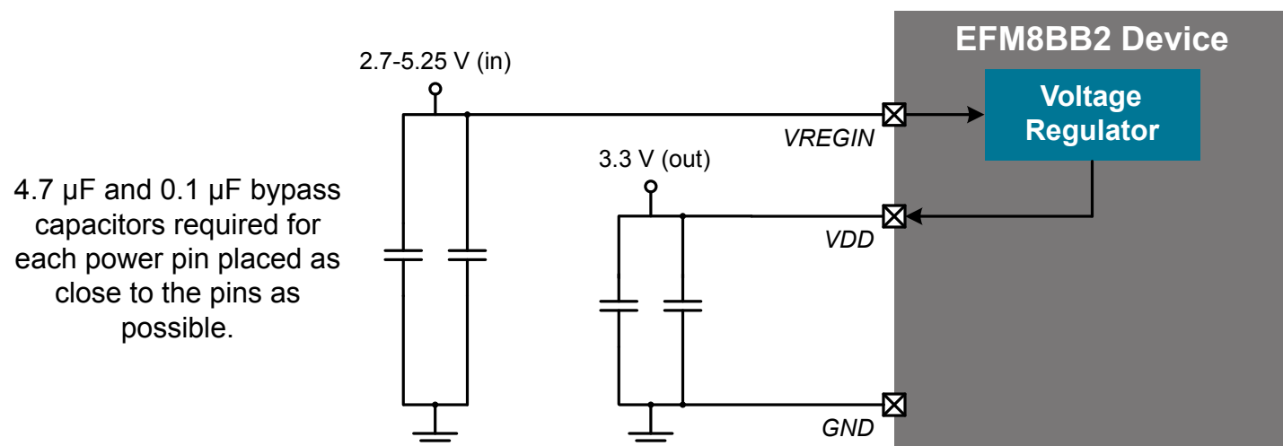
Figure 5.1. Connection Diagram with Voltage Regulator Used
