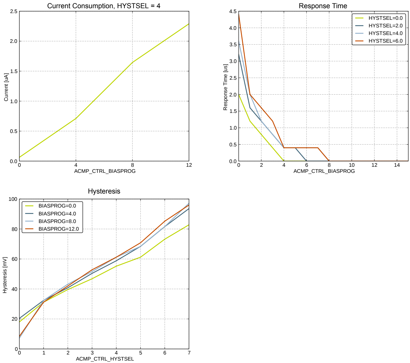
Figure 4.37. ACMP Characteristics, V_{dd} = 3\text{ V} , \text{Temp} = 25\text{ }^{\circ}\text{C} , \text{FULLBIAS} = 0 , \text{HALFBIAS} = 1
