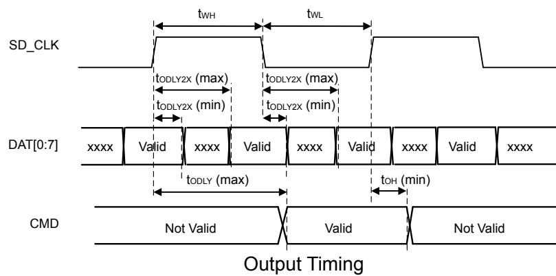
Figure 4.16. SDIO MMC DDR Mode Timing
