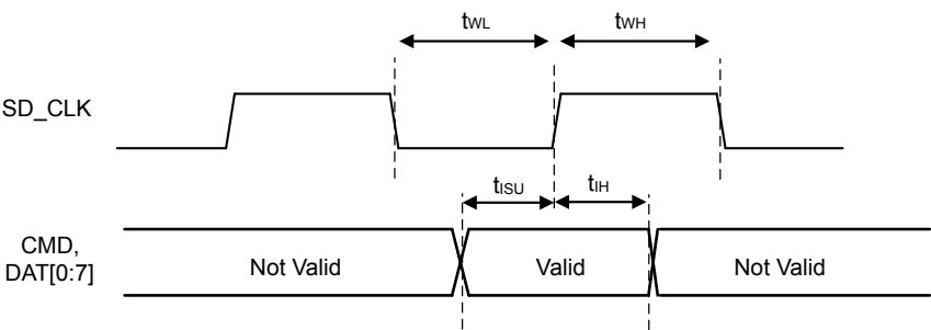
Input Timing
