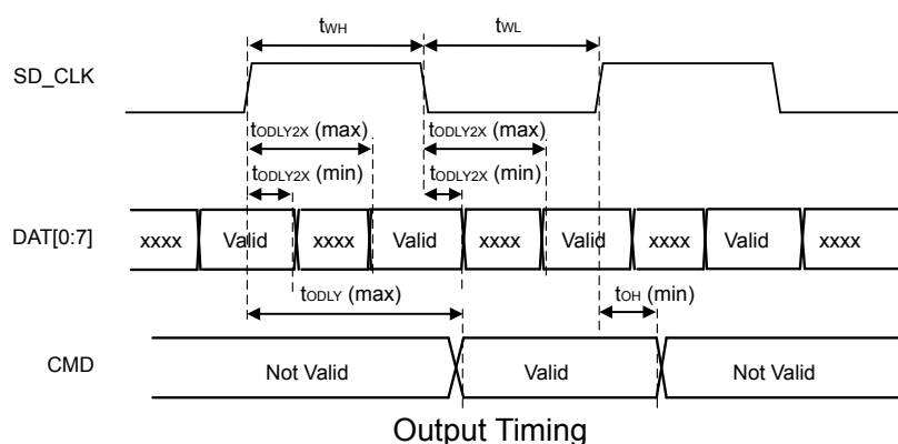
Figure 4.16. SDIO MMC DDR Mode Timing
