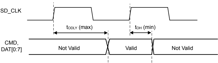
Output Timing
