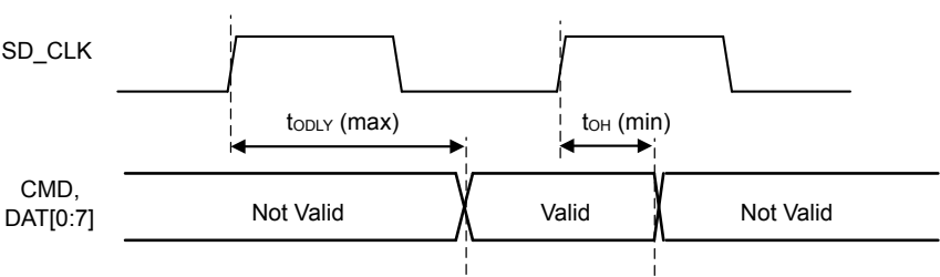
Output Timing
