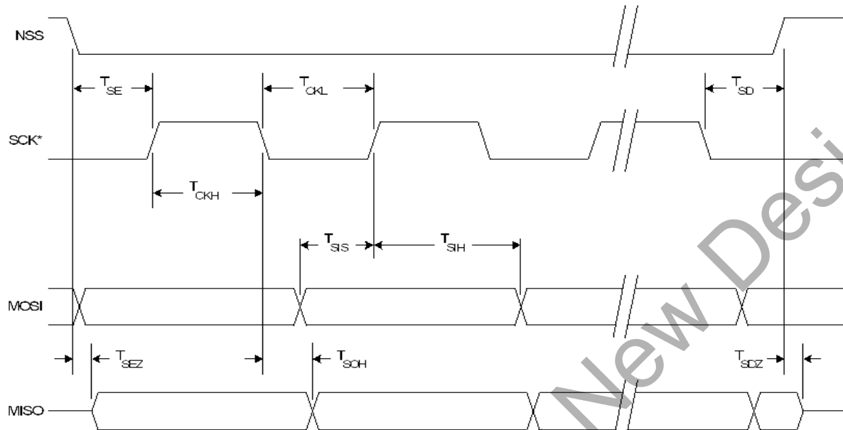
Figure 27.10. SPI Slave Timing (CKPHA = 0)
