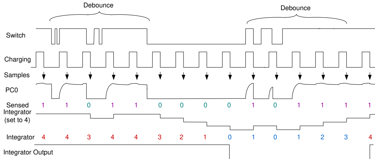
Figure 25.4. Debounce Timing
