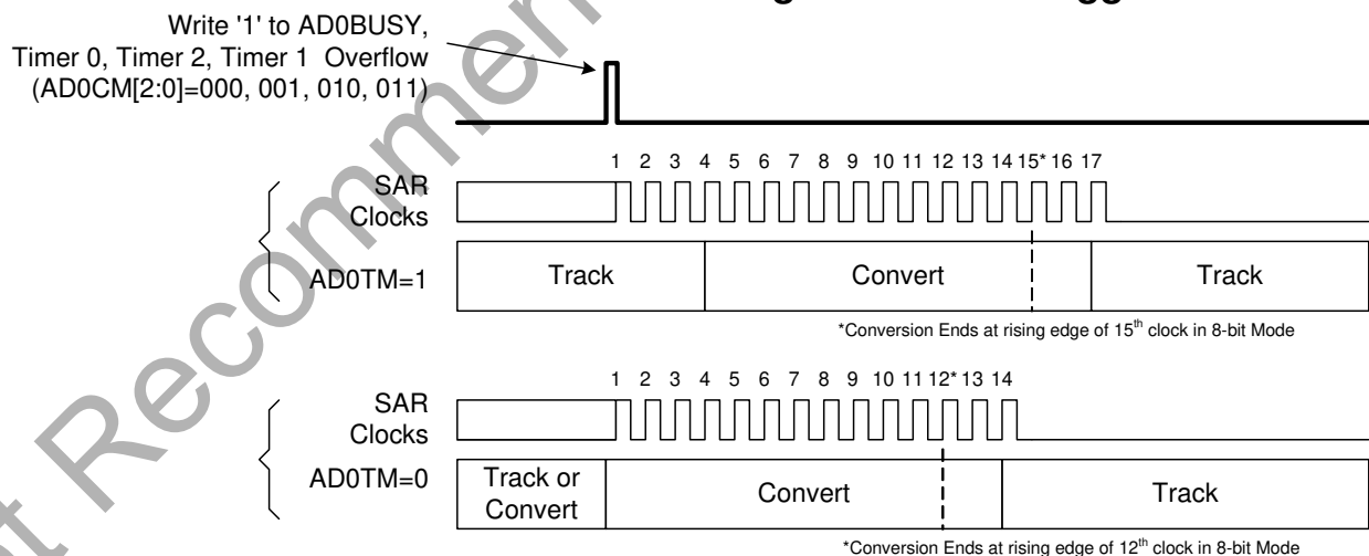
Figure 10.2. 10-Bit ADC Track and Conversion Example Timing
