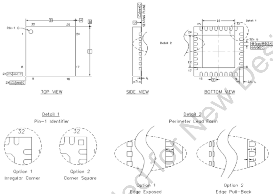
Figure 4.9. QFN-32 Package Drawing
