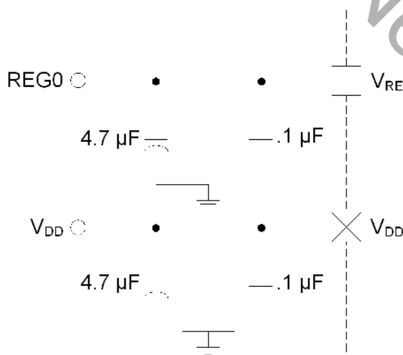
Figure 9.1. External Capacitors for Voltage Regulator Input/Output—Regulator Enabled
