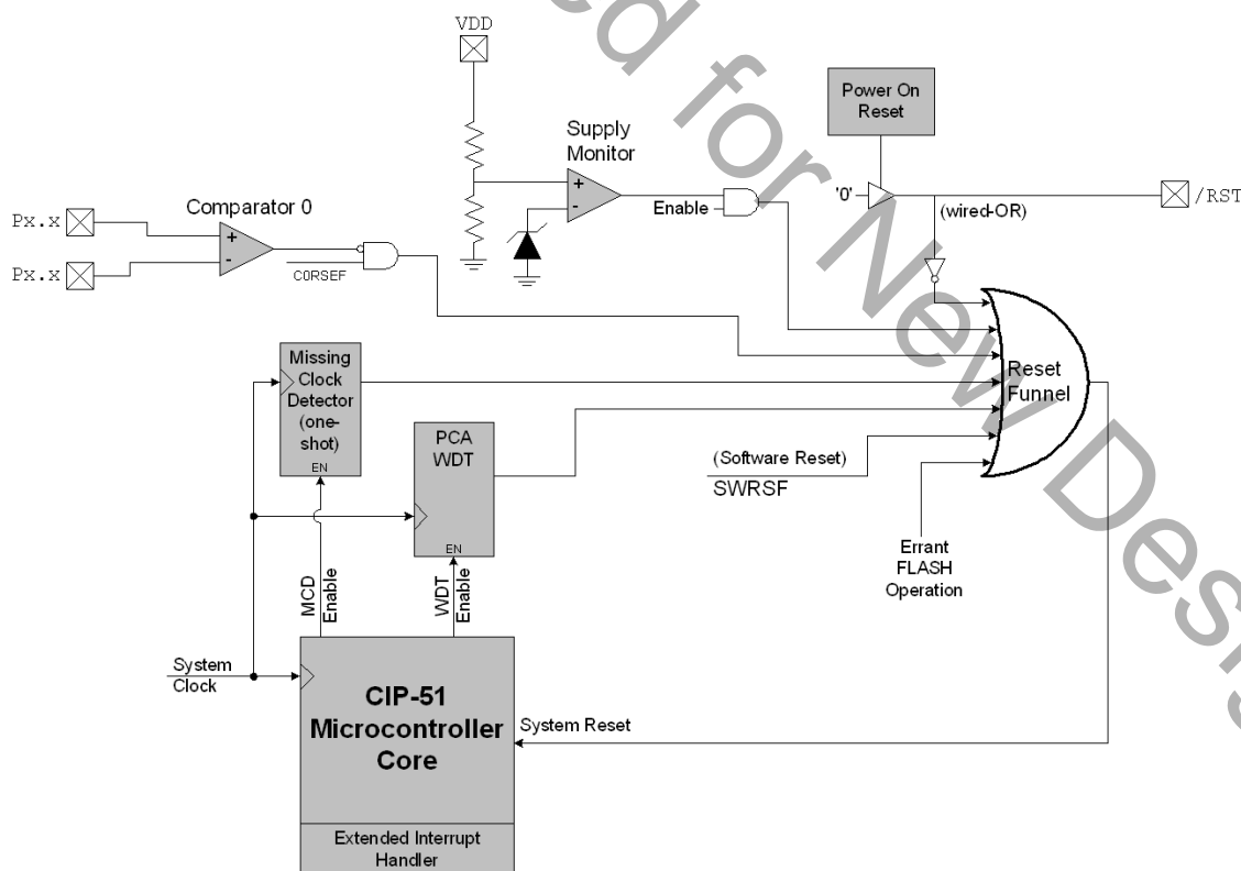
Figure 16.1. Reset Sources
