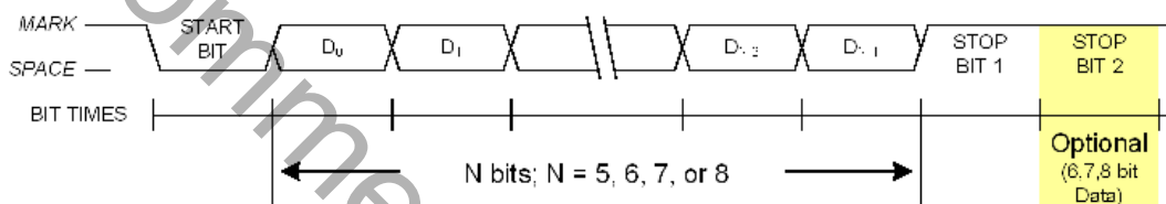
Figure 23.2. UART0 Timing Without Parity or Extra Bit
