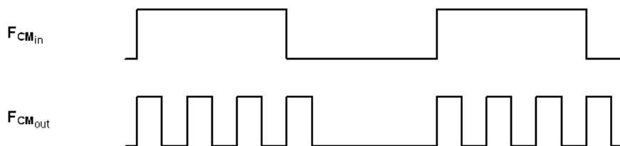
Figure 18.2. Example Clock Multiplier Output
