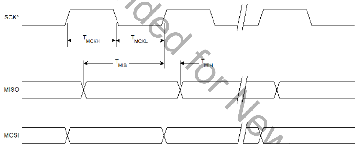
Figure 22.9. SPI Master Timing (CKPHA = 1)
