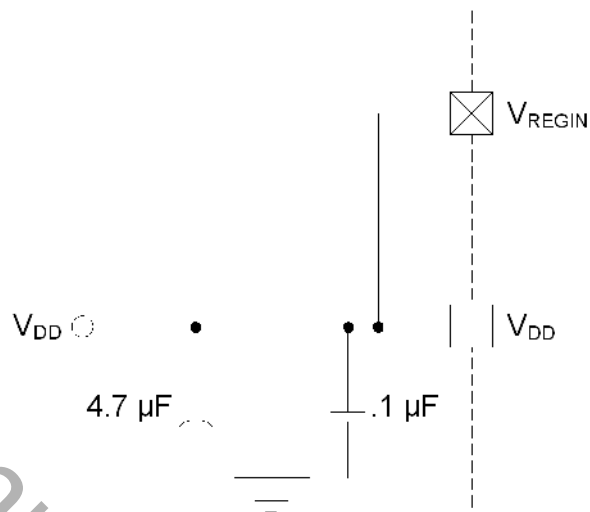
Figure 9.2. External Capacitors for Voltage Regulator Input/Output—Regulator Disabled
