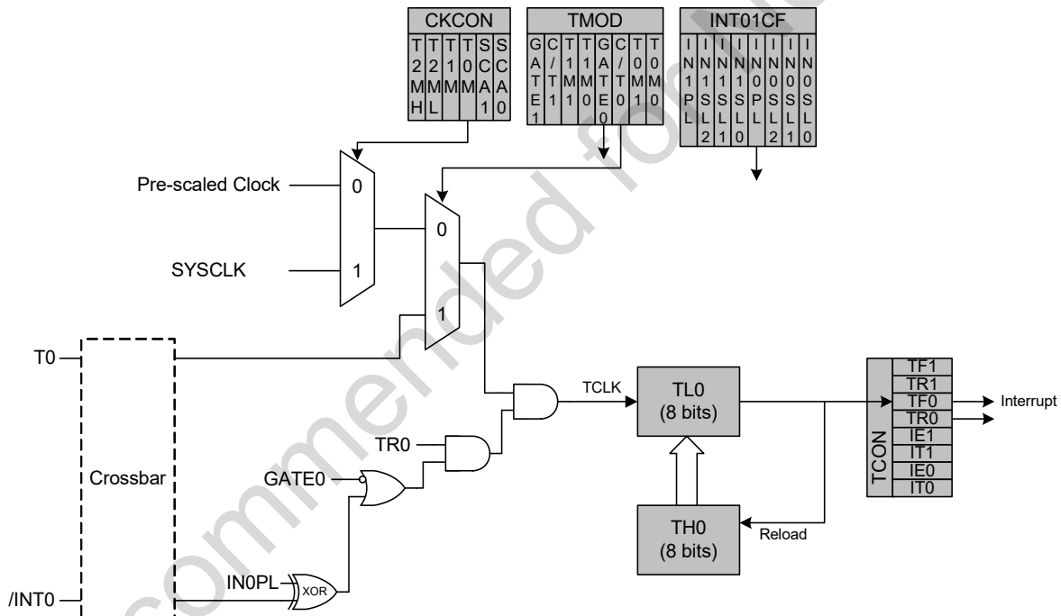
Figure 18.2. T0 Mode 2 Block Diagram
