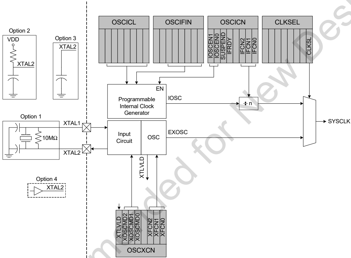
Figure 14.1. Oscillator Diagram
