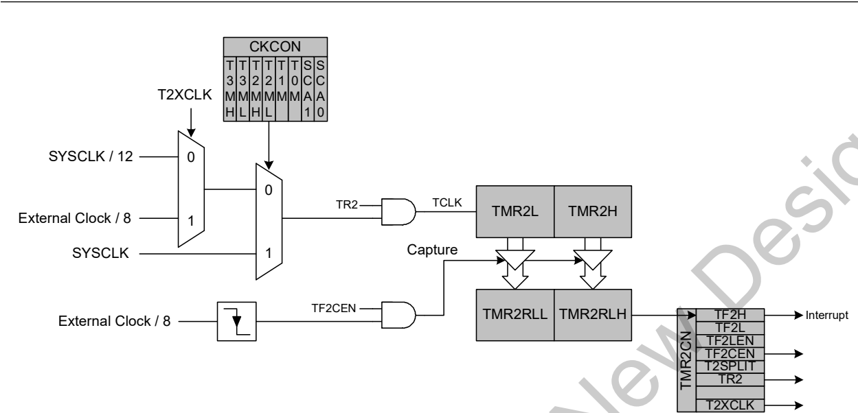
Figure 26.6. Timer 2 External Oscillator Capture Mode Block Diagram
