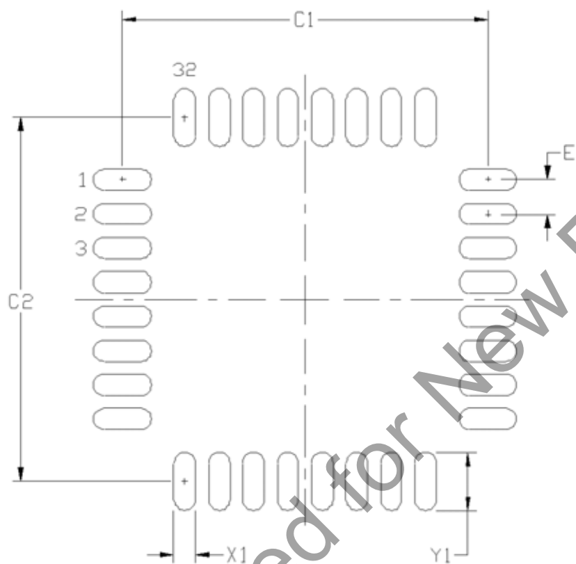
Figure 4.4. LQFP-32 Recommended PCB Land Pattern
