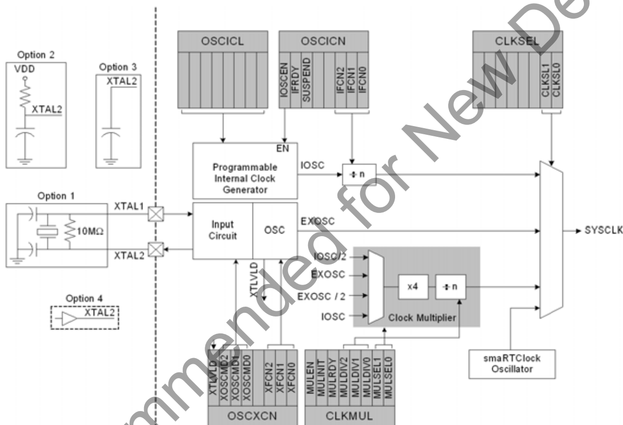
Figure 19.1. Oscillator Diagram
