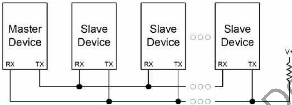
Figure 22.6. UART Multi-Processor Mode Interconnect Diagram
