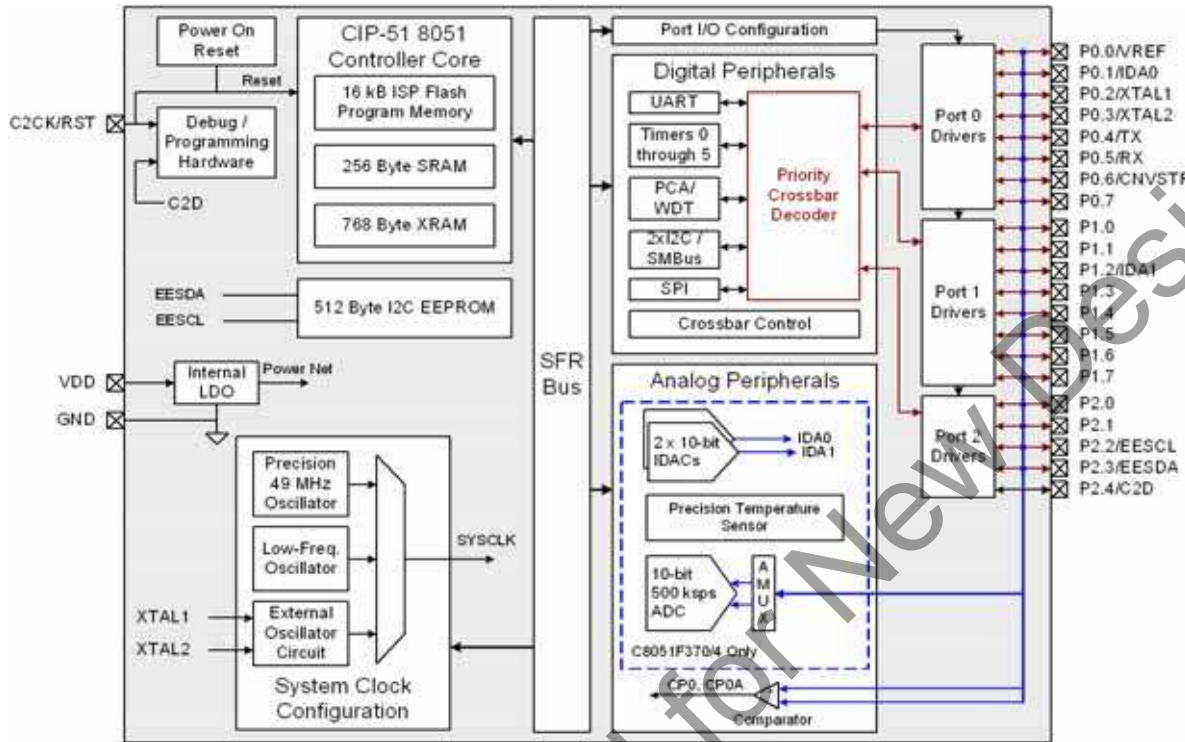
Figure 1.3. C8051F370/1/4/5 Block Diagram
