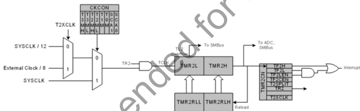
Figure 31.4. Timer 2 16-Bit Mode Block Diagram
