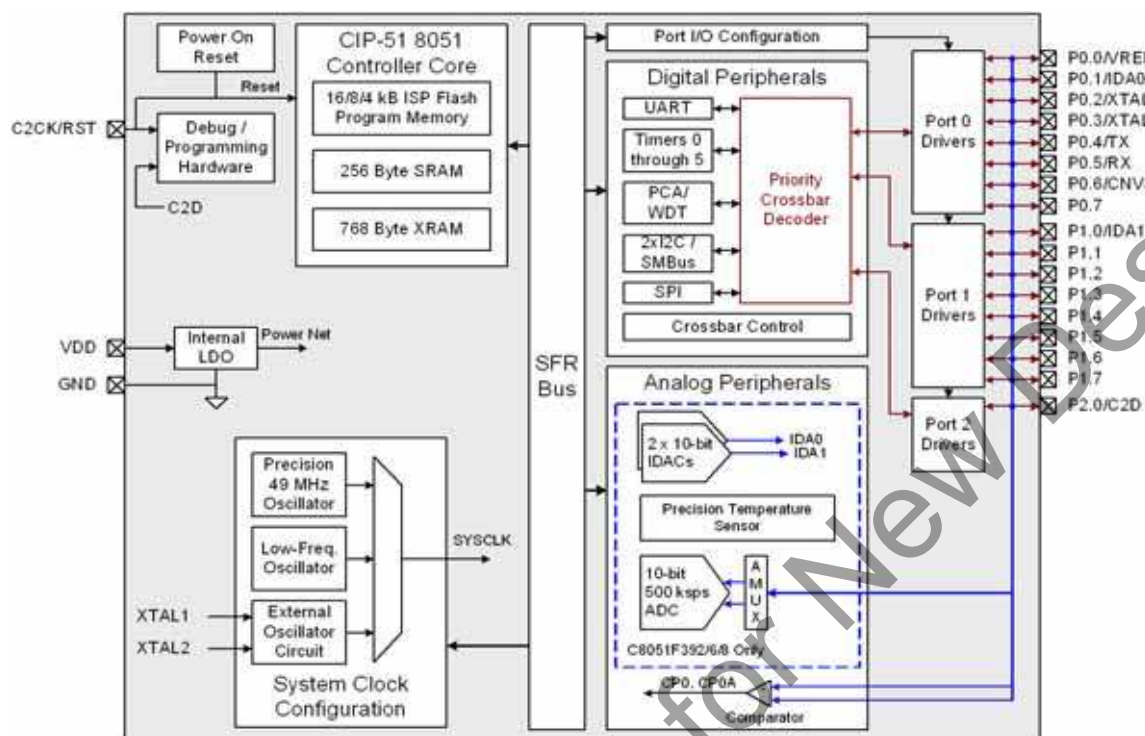
Figure 1.1. C8051F392/3/6/7/8/9 Block Diagram
