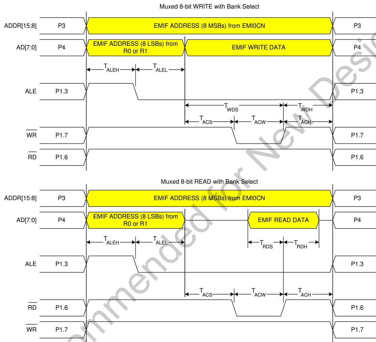
Figure 14.10. Multiplexed 8-bit MOVX with Bank Select Timing
