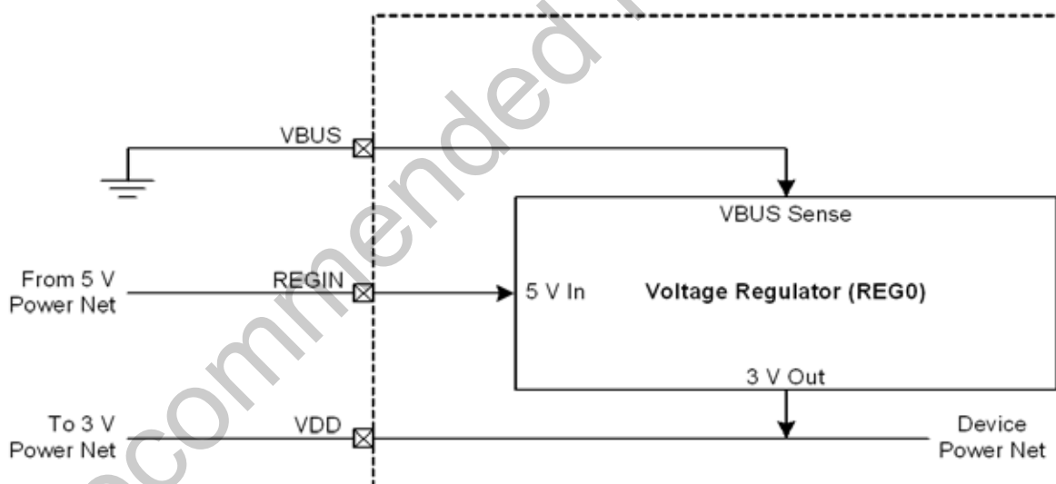
Figure 8.4. REG0 Configuration: No USB Connection
