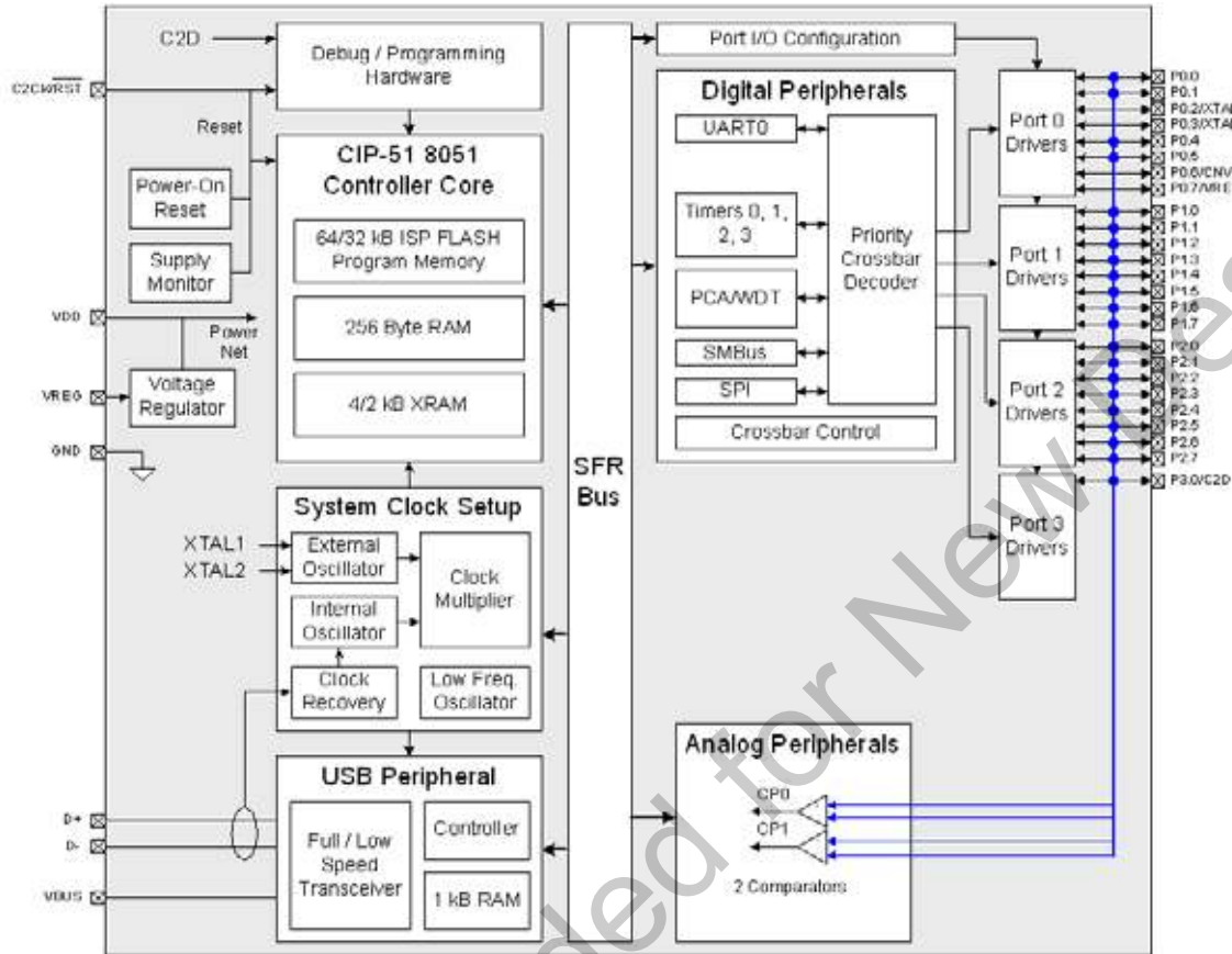
Figure 1.4. C8051F349/D Block Diagram
