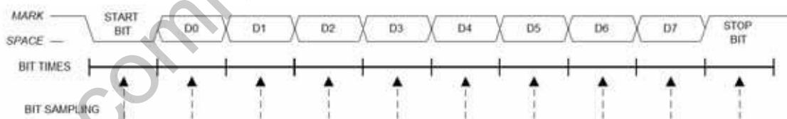
Figure 18.4. 8-Bit UART Timing Diagram
