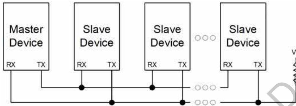
Figure 18.6. UART Multi-Processor Mode Interconnect Diagram
