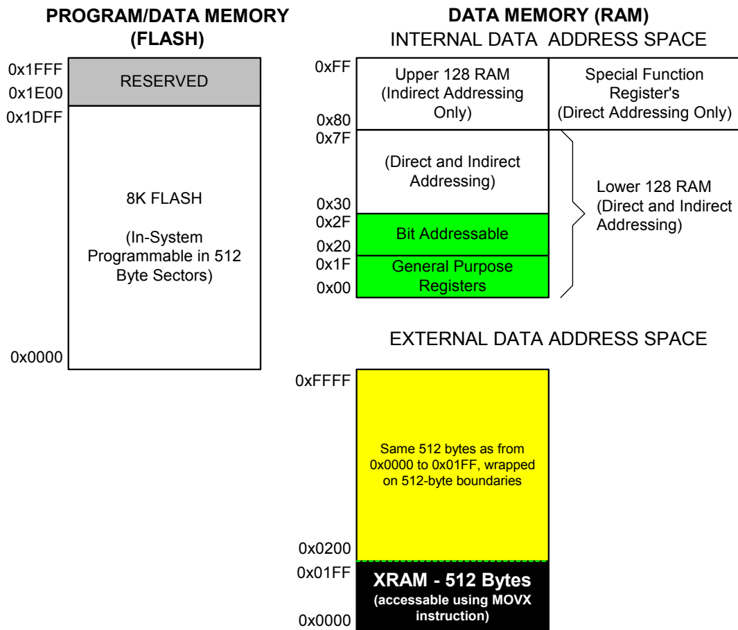
Figure 9.2. Memory Map
