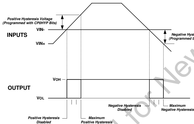
Figure 7.3. Comparator Hysteresis Plot
