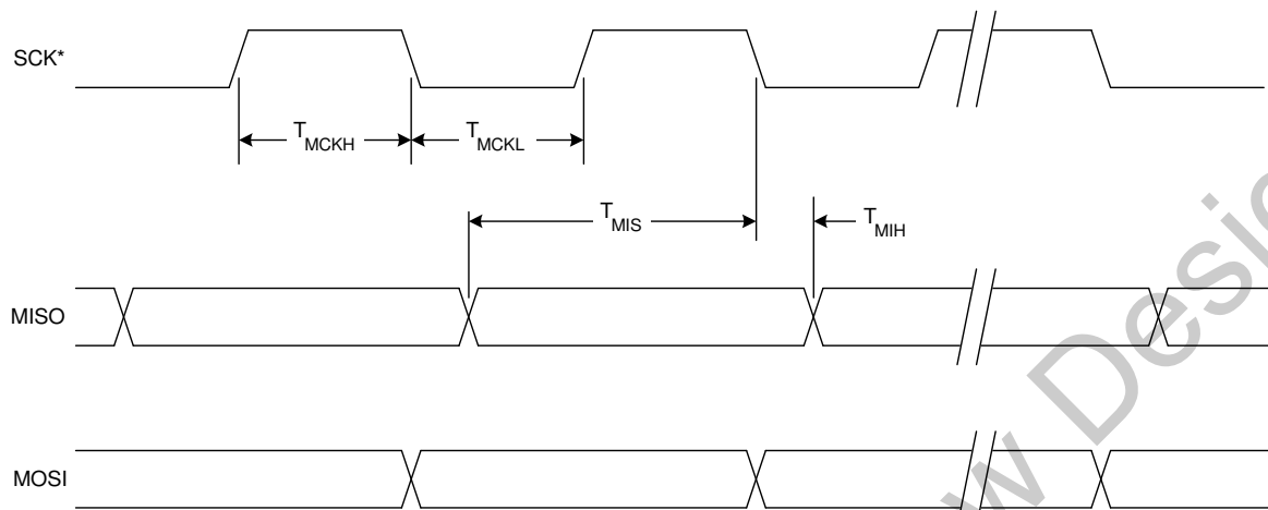
Figure 18.8. SPI Master Timing (CKPHA = 0)
