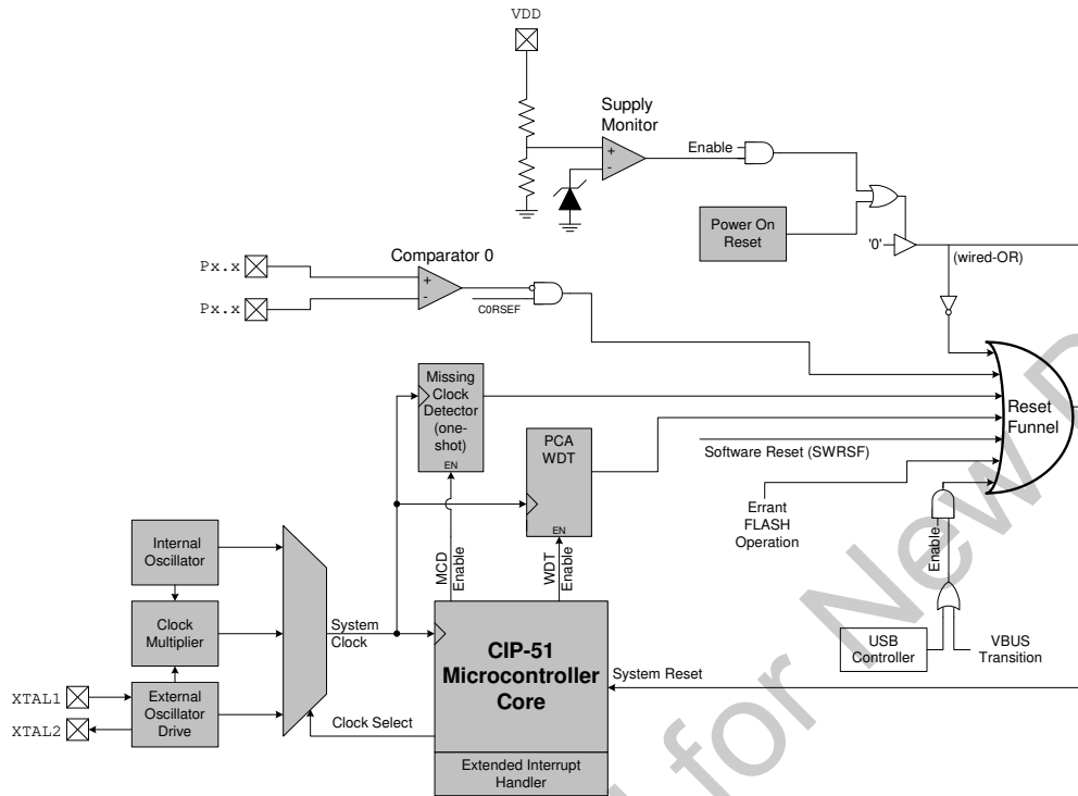
Figure 1.3. On-Chip Clock and Reset
