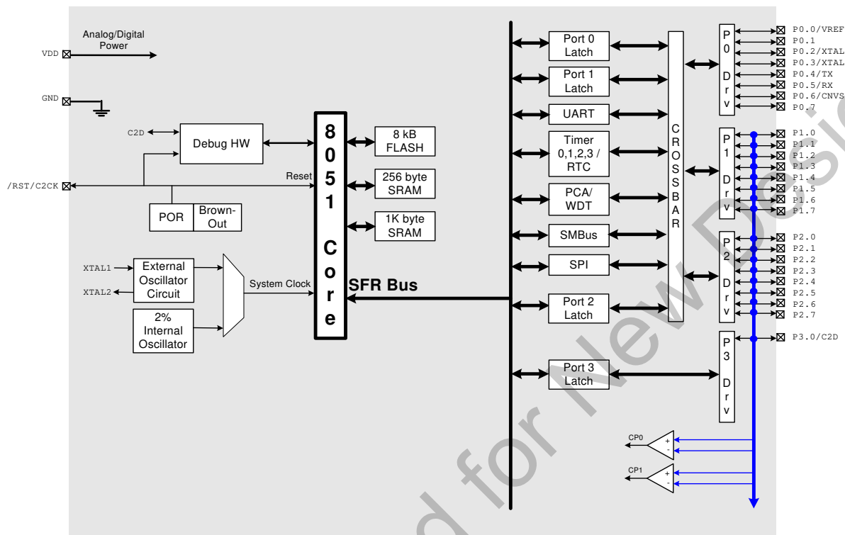
Figure 1.6. C8051F315 Block Diagram
