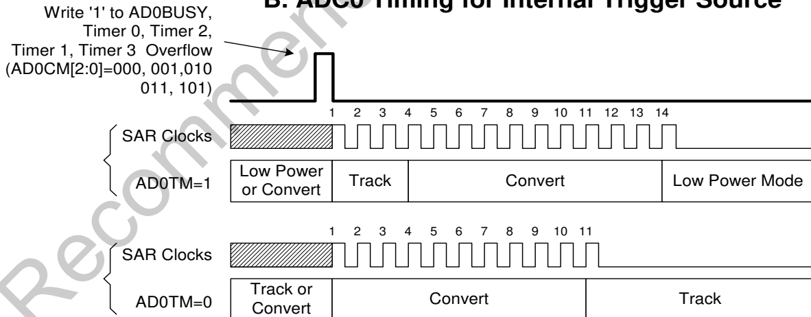
Figure 5.4. 12-Bit ADC Track and Conversion Example Timing
