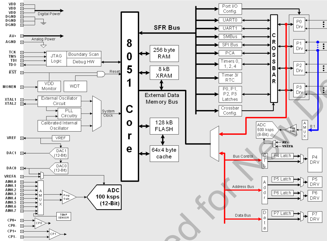
Figure 1.2. C8051F121/125 Block Diagram
