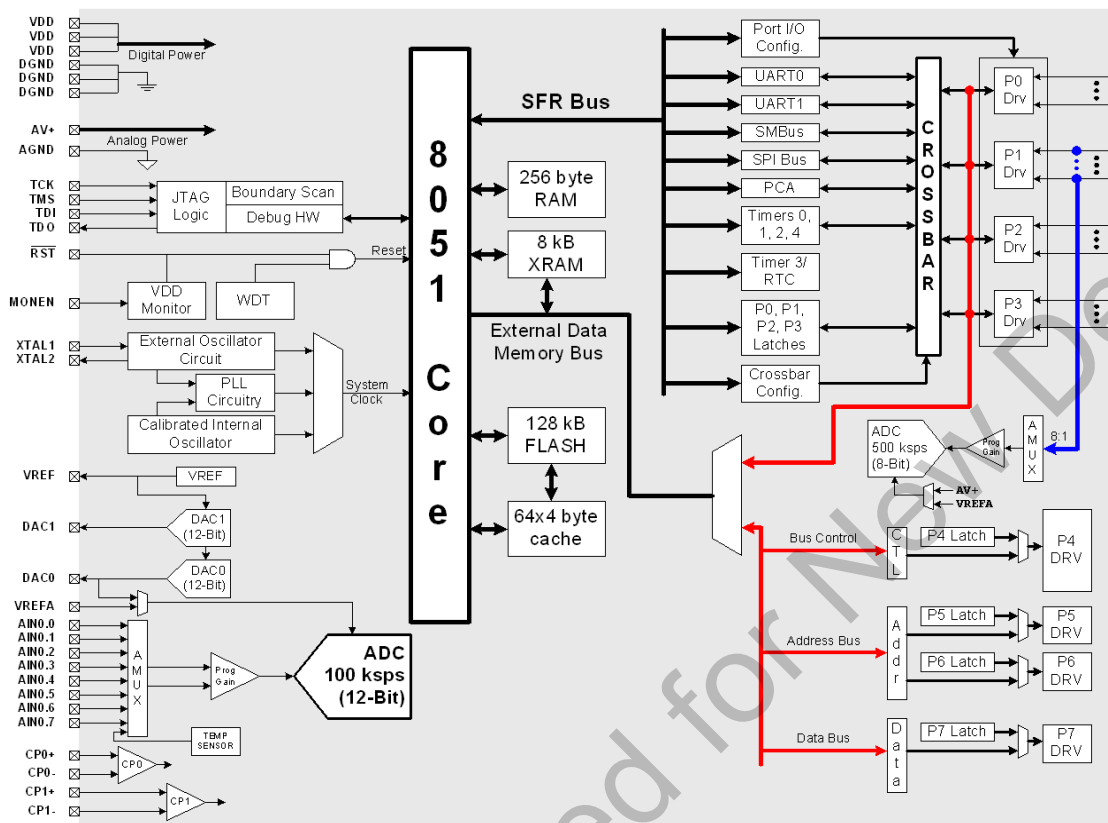
Figure 1.2. C8051F121/125 Block Diagram
