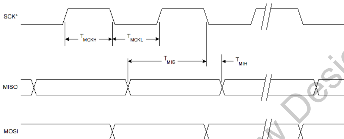
Figure 20.8. SPI Master Timing (CKPHA = 0)
