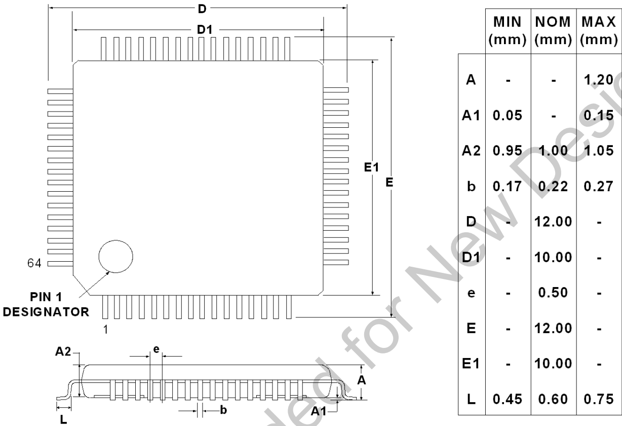
Figure 4.6. TQFP-64 Package Drawing
