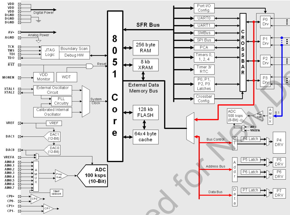
Figure 1.4. C8051F123/127 Block Diagram
