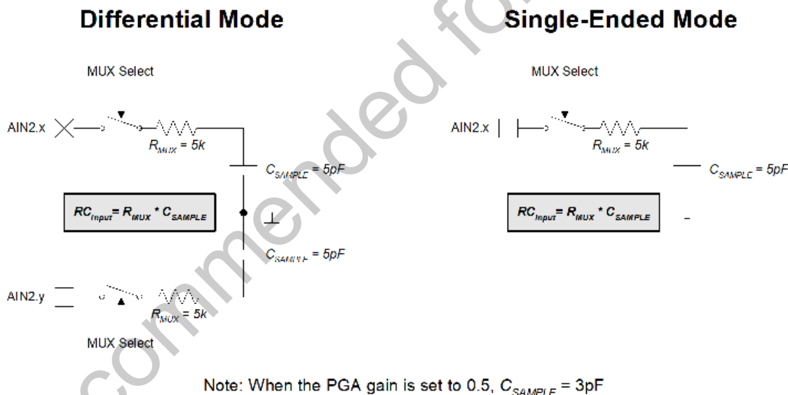
Figure 7.3. ADC2 Equivalent Input Circuit
