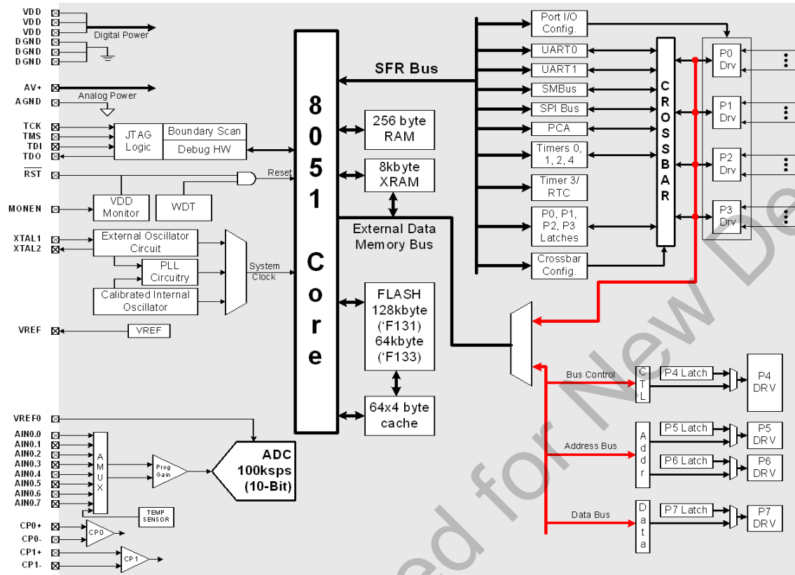
Figure 1.6. C8051F131/133 Block Diagram
